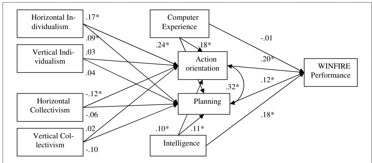
Figure 1: Path analysis indicating relationships among all variables in WINFIRE.
