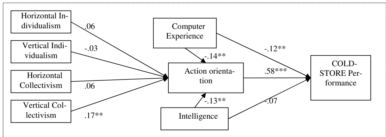
Figure 2: Path analysis indicating relationships among all variables in COLDSTORE.
