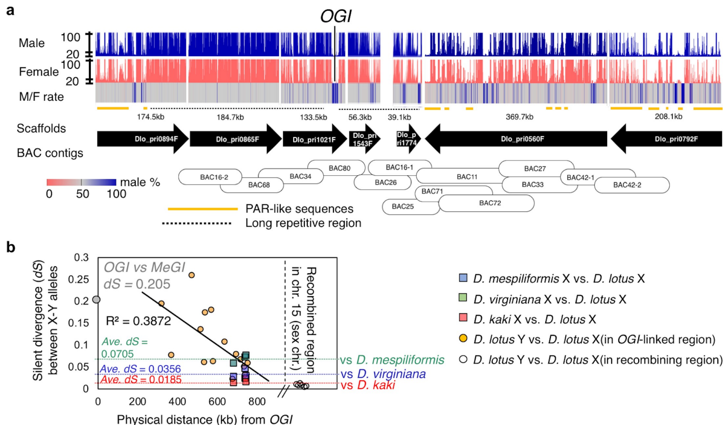
Fig 6. Genomic context of the Y-chromosomal region surrounding OGI. a, Read coverage from male (blue) and female (pink) samples and male/female coverage ratio across the scaffolds covering the male-specific region of the Y-chromosome. For both the male and female reads, expected coverage a single-copy sites is approximately 20 (grey lines across). This male-specific region was assembled via anchoring of the scaffolds with BAC sequences. Approximately 1.3Mb region was covered by Y-allelic scaffolds. More than 400kb of long repetitive sequences (dotted lines), flank OGI. Outer regions of these hyper repetitive sequences contain male-specific sequences (blue bands in M/F rate) and pseudo autosomal region (PAR)-like sequences (orange lines), where M/F rate was less than 70%, and the percentage of repetitive sequences was much lower. b, The silent divergence rate (dS) between X and Y alleles of the genes located in the PAR-like sequences (orange circles) decreases with distance to OGI. Still, for most of these genes, the dS value between the X and Y alleles was larger than the average interspecific dS between the X alleles of D. lotus and D. mespiliformis (green square and dotted line), D. lotus and D. virginiana (blue square and dotted line), and D. lotus and D. kaki (red square dotted line). These results suggest that, in these PAR-like sequences, recombination between the X and Y alleles was suppressed before the divergence of Diospyros species, or at least predates the divergence between D. lotus and D. kaki . dS values for genes located in the regions closest to OGI are comparable to dS values between OGI and MeGI (gray circle, dS = 0.205), which suggest that little or no recombination occurred between these sequences after the establishment of OGI. In comparison, dS values between the X and Y alleles of genes located in the recombining region of chromosomes 15 are much lower (white circles on the right).
