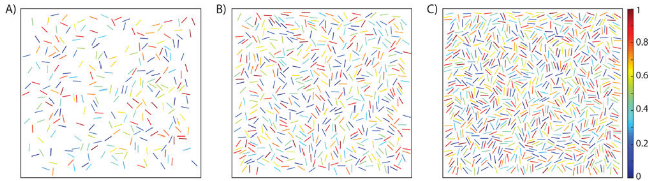
FIG. 4. Initial cell distributions in simulations of the populations with densities 6.4% (A), 12.8% (B) and 20% (C). The size of simulation domain is set to 100 \times 100 \mu\text{m}^2 and the length of cells is 5 \mu\text{m} . The color scale shows the level of the protein on each cell that is chosen randomly from a uniform distribution from [0, 1] .
