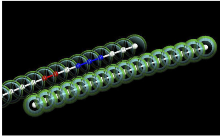
FIG. 6. Representation of cells with SCEs. White spheres and segments indicate positions and bonds of SCEs. The green (outer) shell represents the boundary for the zone of attraction, the cyan (inner) shell represents the boundary of the repulsive force. (Repulsion and attraction zones are not to exact scale). Red SCEs highlight stretching interactions between SCEs. Blue SCEs represent the bending interaction between SCEs.
