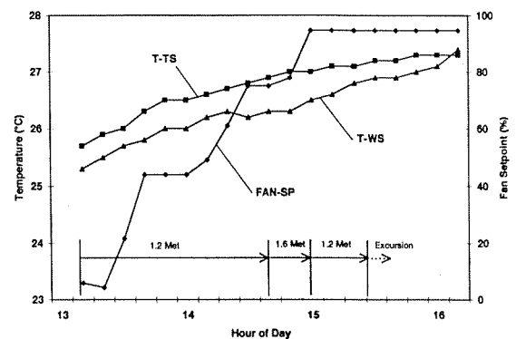
Figure 7 Comparison of Thermostat (T-TS), Workstation (T-WS) temperatures and fan setpoint for Test 4 (Subject ID #6)
