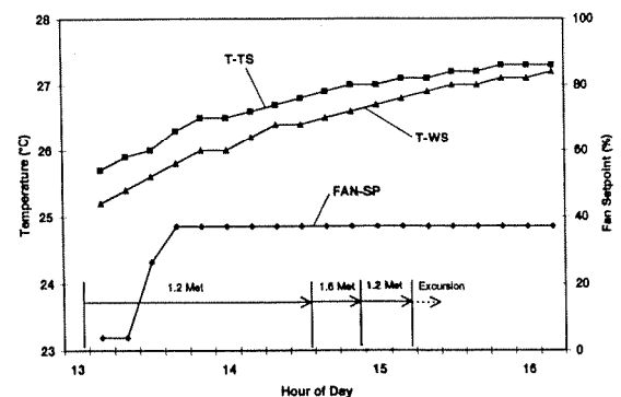
Figure 8 Comparison of Thermostat (T-TS), Workstation (T-WS) temperatures and fan setpoint for Test 4 (Subject ID #7)
