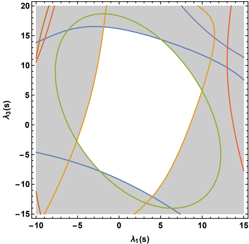
Figure 5: Limits on \lambda_1(s) and \lambda_3(s) in the MSSM-like 2HDM due to unitarity, |a_0 - i/2| \leq 1/2 . The blue, orange, green, red, purple, and brown curves correspond to a_0^{11\text{odd}} , a_{0+}^{00\text{even}} , a_{0-}^{00\text{even}} , a_{0-}^{00\text{even}} , a_0^{01\text{odd}} , and a_0^{01\text{even}} respectively.
