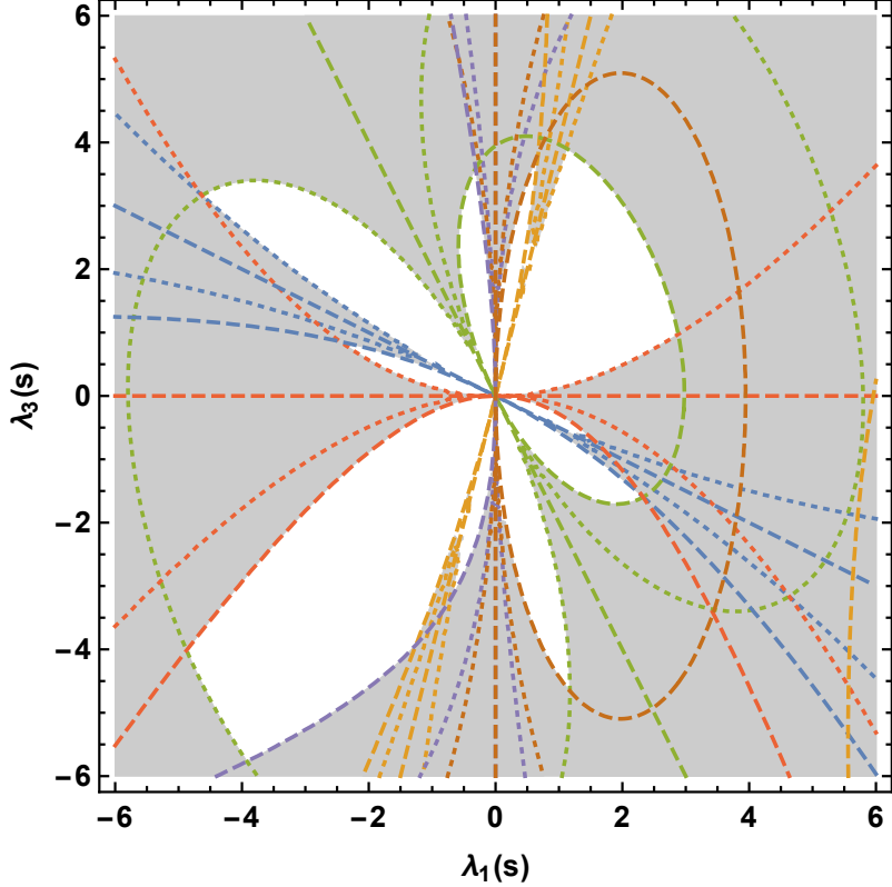
Figure 6: Limits on \lambda_1(s) and \lambda_3(s) in the MSSM-like 2HDM due to perturbativity, R_1 , R'_1 . The colors of the curves correspond to the same eigenvalues as they did in Fig. 5.
