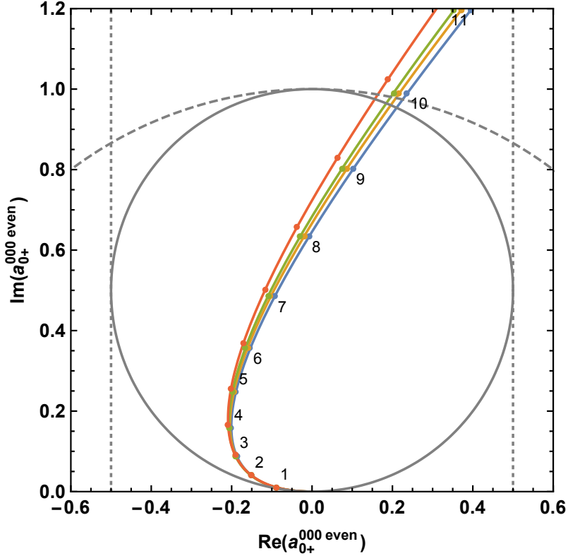
Figure 2: Argand diagram of a_{0+}^{000 \text{ even}} in the SO(3) symmetric 2HDM as a function of the running coupling \lambda_1(s) . The blue and red curves corresponds to m_h^2 = m_A^2 and m_h^2 = 8m_A^2 respectively, and are labeled with various values of \lambda_1(s) . The orange curve is the limit s \gg m_A^2 \gg m_h^2 . Finally, the green corresponds to the contribution of the 1PI diagrams alone. The solid circle is the bound |a_0 - i/2| \leq 1/2 , whereas the dashed arc and the dotted vertical lines represent the bounds |a_0| \leq 1 and |\text{Re}(a_0)| \leq 1/2 respectively.
