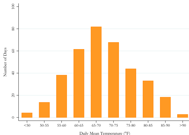
Fig. 2. Daily mean temperature, weighted by population.
