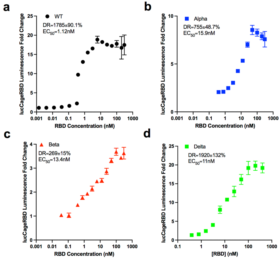
Extended Data Fig. 3 | Detection of RBD strains by lucCageRBD. a-d, Fold change increase in luminescence from different concentrations of RBD WT ( a ), Alpha ( b ), Beta ( c ), Delta ( d ) tested in the lucCageRBD assay. All experiments were performed in triplicates and data are mean \pm s.e.m.
