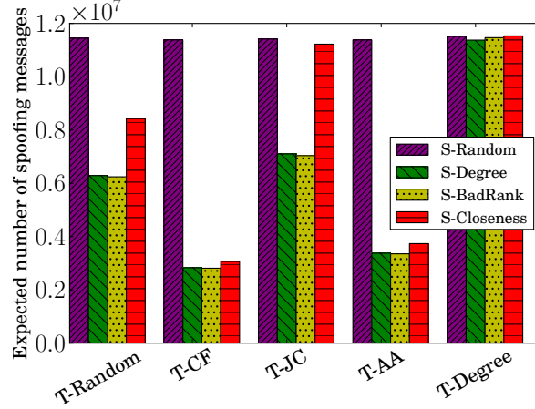
Figure 2.4: The expected number of required spoofing messages for different seed users selection strategies and trustee selection strategies on Flickr. We observe that our strategy T-Degree can increase the attacker's costs by a few times in some cases.
