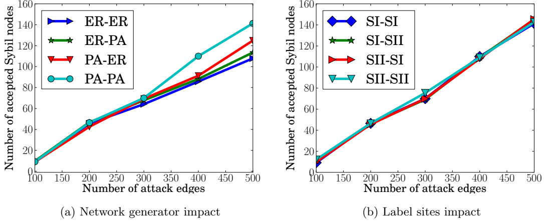
Figure 3.3: The accepted Sybil nodes as a function of the number of attack edges. (a) Impact of different network generators. The notation M1 - M2 means we use M1 to produce the benign region and M2 to synthesize the Sybil region. We observe that the attackers should design their Sybil regions to approach scale-free networks in order to inject more Sybils. (b) Impact of different combinations of label sites. Our algorithm SybilBelief is robust to label sites.
