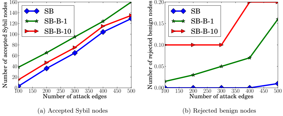
Figure 3.7: Boosting with only labeled benign nodes. The numbers in the legend are the number of boosting trials. With only labeled benign nodes, SybilBelief (SB) with boosting can achieve performances comparable to the case where both benign and Sybil labels are observed. Furthermore, the number of boosting trials balances between the accepted Sybil nodes and rejected benign nodes.
