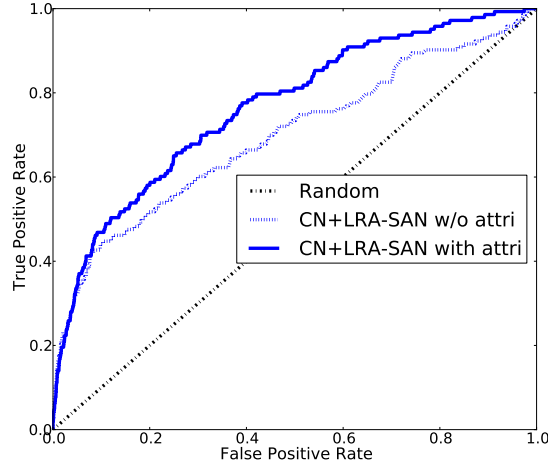
Figure 4.3: ROC curves of the CN+LRA-SAN algorithm for predicting new links. AUG4-SEP4 is the train-test pair. JUL4-AUG4 is the train-validation pair.
