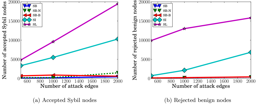
Figure 3.8: The number of accepted Sybil nodes and rejected benign nodes as a function of the number of attack edges. The benign region is the Facebook network, and the Sybil regions are synthesized by PA model. We observe that SB, SB-N, and SB-B all work an order of magnitude better than previous classification systems. Furthermore, we find that incorporating both benign and Sybil labels increases the performance of our algorithm.
