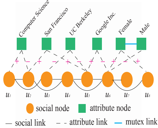
Figure 4.1: Illustration of a Social-Attribute Network (SAN). The link prediction problem reduces to predicting social links while the attribute inference problem involves predicting attribute links.
