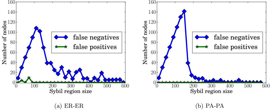
Figure 3.2: The false negatives and false positives as a function of the Sybil region size. (a) Networks are synthesized by the ER model. (b) Networks are synthesized by the PA model. There exists an optimal strategy for the attackers.
