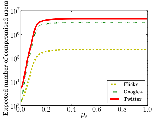
(c) Impact of p_s
