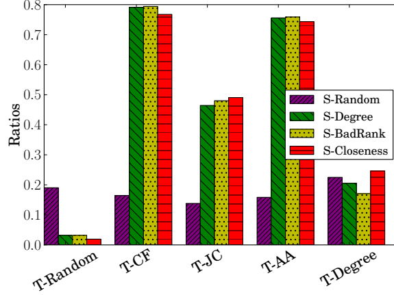
Figure 2.5: The ratios between the expected number of users that are compromised without spoofing attacks and those with spoofing attacks for different seed selection strategies and different trustee selection strategies on Flickr. We find that the expected number of compromised users only decreases by 20% to 25% when the attacker does not use spoofing attacks in some cases, which implies that spoofing attacks are optional.
