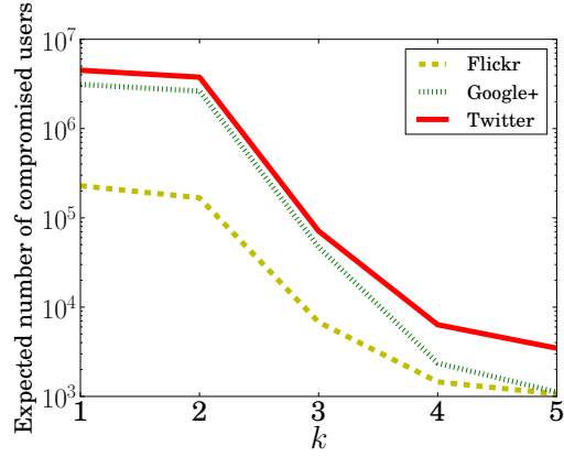
(b) Impact of k
