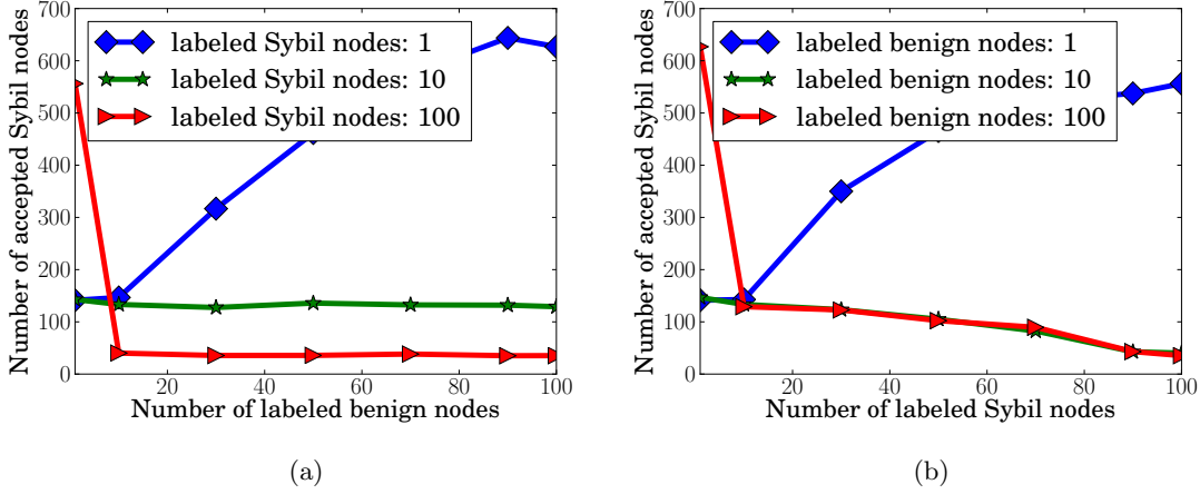
Figure 3.5: The number of accepted Sybil nodes as a function of the number of labeled benign and Sybil nodes. (a) The number of Sybil nodes is fixed while varying the number of benign labels. (b) The number of labeled benign nodes is fixed while increasing the number of Sybil labels. We observe that SybilBelief only requires one label per community.
