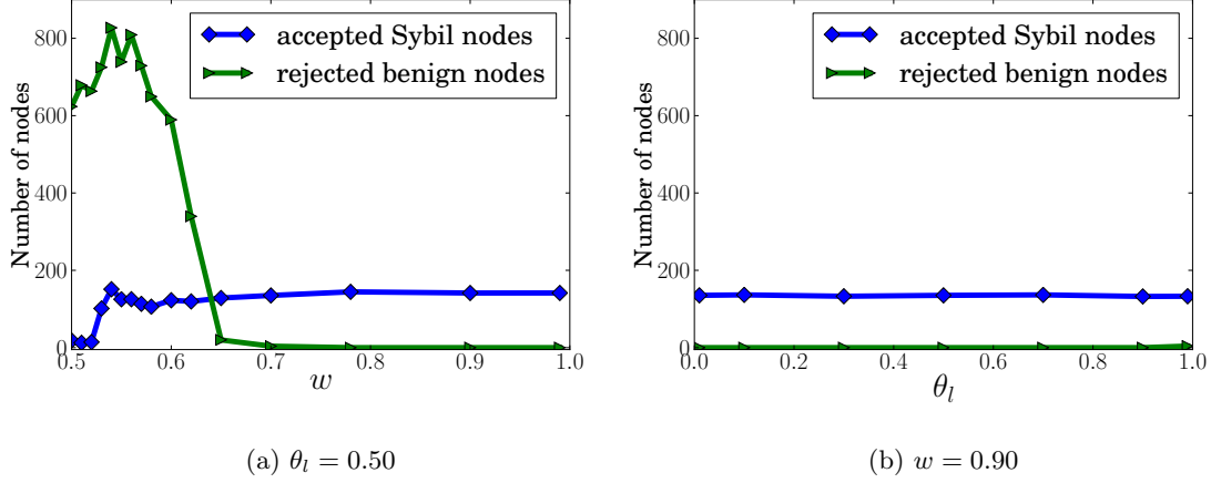
Figure 3.4: The number of accepted Sybil nodes and rejected benign nodes as a function of the model parameters w and \theta_l . (a) \theta_l = 0.50 and we vary w . (b) w = 0.90 and we vary \theta_l . We observe that there exists a phase transition point w_0 (e.g., w_0 \approx 0.65 in our experiments) for the parameter w . SybilBelief is robust for w > w_0 . Moreover, we confirm that SybilBelief performance is independent with \theta_l once it's bigger than 0.
