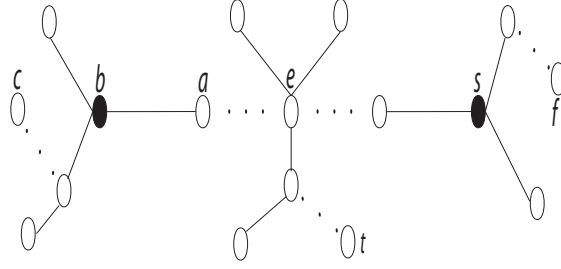
Figure A.1: Illustration of a Pairwise Markov Random Fields on a tree.
