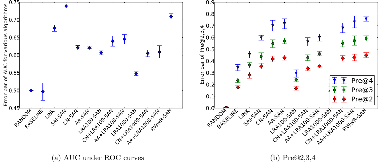
Figure 4.5: Performance of various algorithms on attribute inference on SEP4. (a) AUC under ROC curves. (b) Pre@2,3,4.
