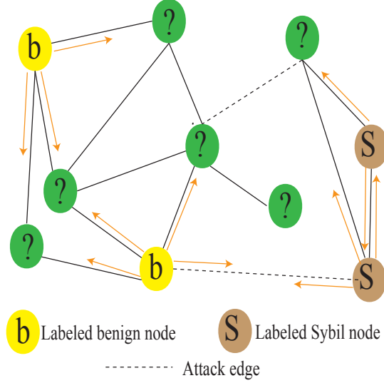
Figure 3.1: The propagation in SybilBelief. Given a set of labeled nodes, we want to infer the labels of the remaining nodes. SybilBelief iteratively propagates the label information from the labeled nodes to their neighbors.
