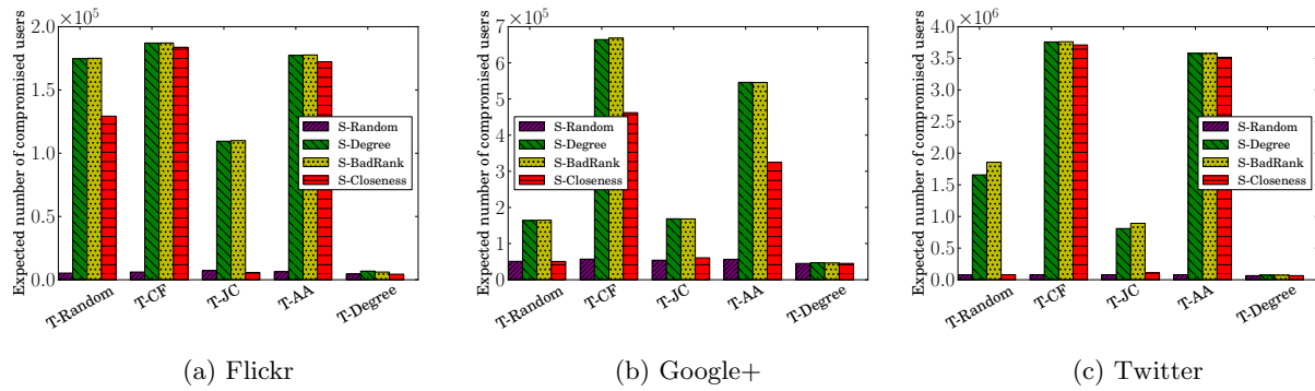
Figure 2.3: The expected number of compromised users for different seed users selection strategies and trustee selection strategies. We find that, with 1,000 seed users, an attacker can compromise two to three orders of magnitude more users with low costs of sending spoofing messages in some cases. However, our strategy T-Degree can decrease the expected number of compromised users by one to two orders of magnitude.
