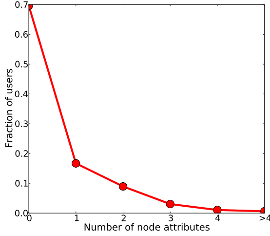
Figure 4.2: The fraction of users as a function of the number of node attributes in the Google+ social network.
