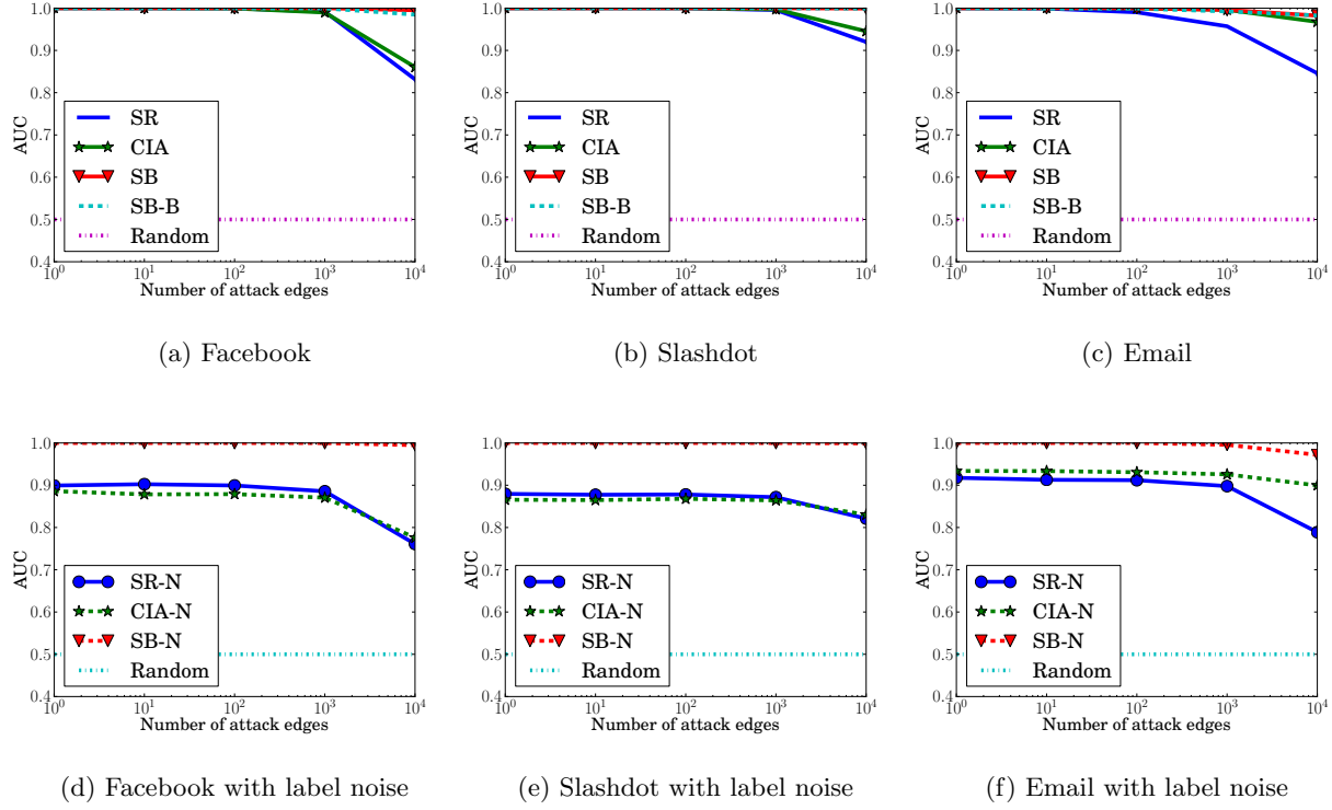
Figure 3.9: AUC as a function of the number of attack edges on different social networks. For each social network, we treat it as both the benign and Sybil regions, and add attack edges between them uniformly at random. The AUCs are averaged over 10 trials for each number of attack edges. We observe that both SB and SB-B outperform previous approaches. Furthermore, in contrast to previous approaches, SB is robust to label noise.
