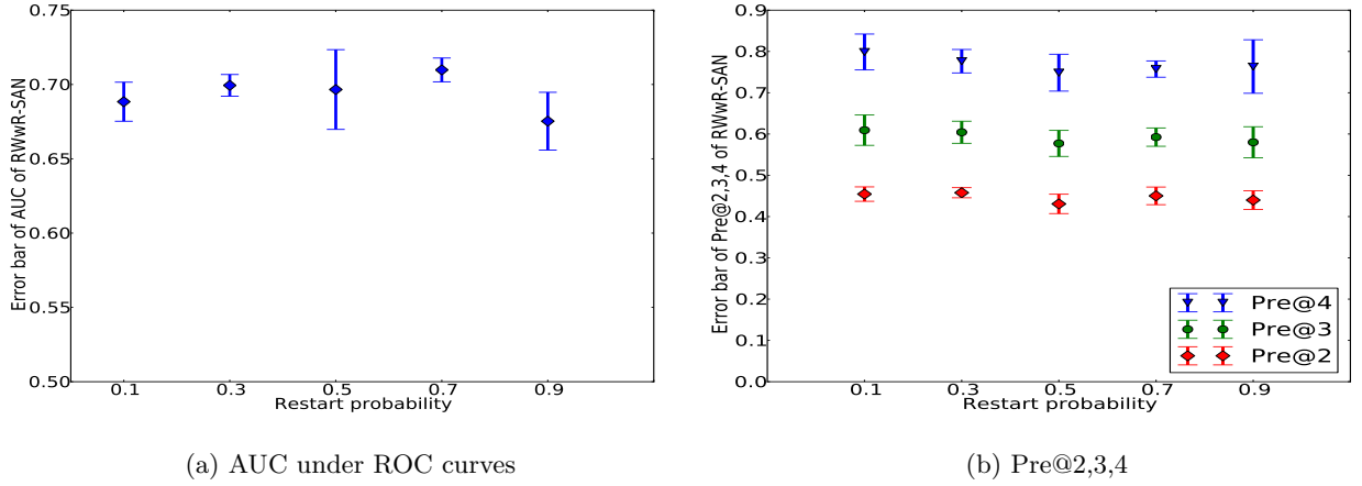
Figure 4.4: Impact of the restart probability on the performance of RWwR-SAN for attribute inference on SEP4. (a) AUC under ROC curves. (b) Pre@2,3,4.
