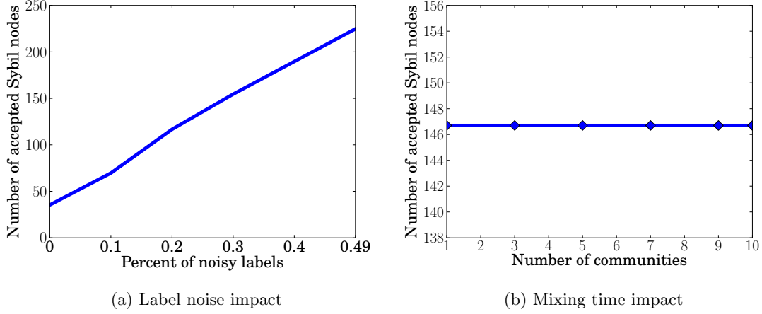
Figure 3.6: Impact of label noise and community structure of the benign region on the number of accepted Sybil nodes. (a) We have 100 labeled benign and Sybil nodes. The x-axis is the percent of both noisy benign and Sybil labels. We find that SybilBelief can tolerate 49% of labels to be incorrect. (b) The benign region consists of multiple communities. We observe that SybilBelief is robust to community structures.
