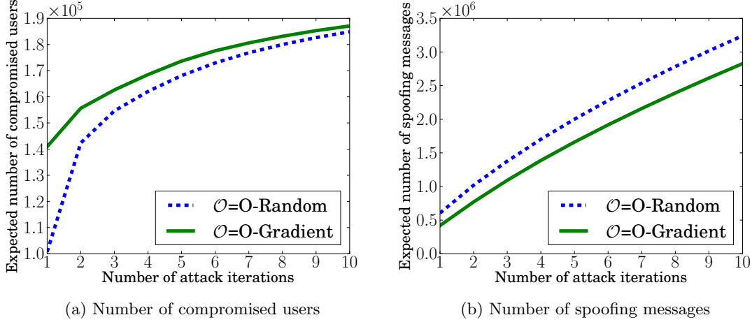
Figure 2.2: Impact of attackers' resources and attack orderings on Flickr. First, we find that an attacker can perform forest fire attacks with low costs. Second, we find that O-Gradient compromises more users and requires fewer spoofing messages than O-Random when the attacker performs a given number of attack iterations.
