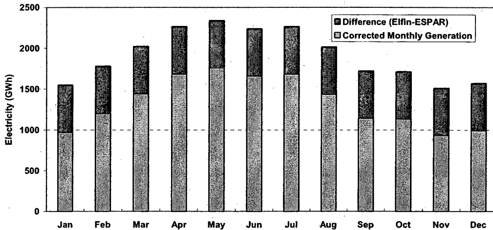
Figure 3. Corrected 1990 Monthly Hydro Generation for PG&E
