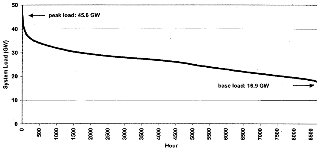
Figure 8. 1999 CAISO Load Duration Curve
