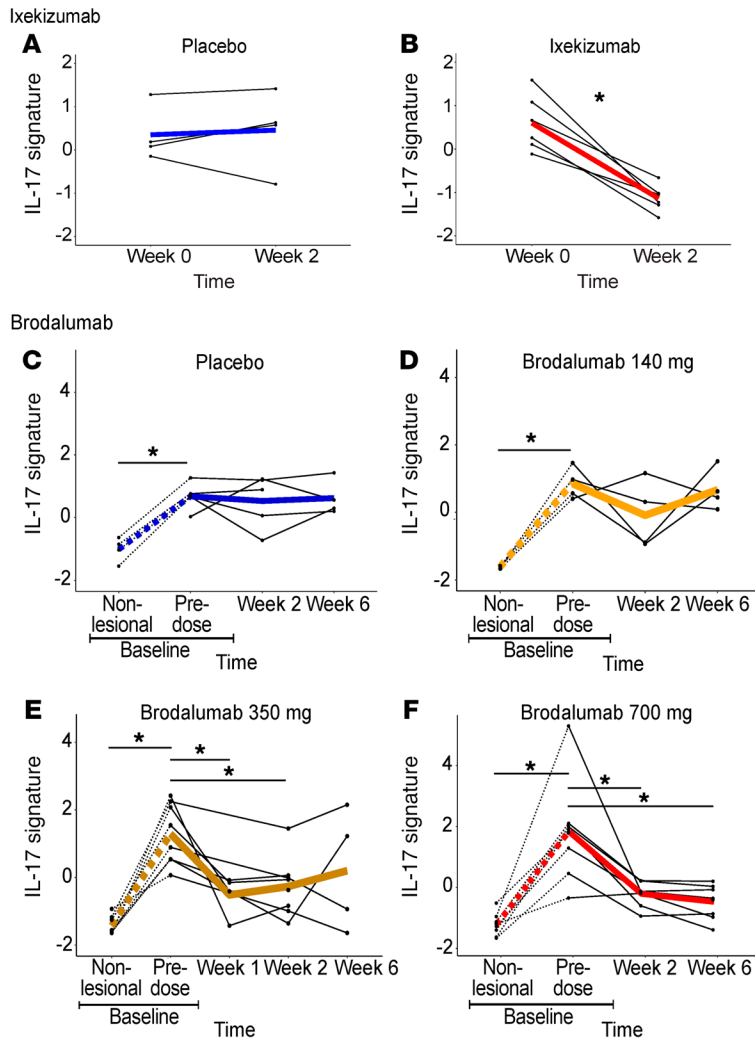
Figure 3. IL-17 blockade in psoriasis. Ixekizumab: compared with placebo (A) (n = 4), the IL-17 signature was decreased in psoriatic lesions (n = 6) after 2 weeks of ixekizumab (B). (C–F) Brodalumab: Compared with placebo (C) (n = 5), brodalumab (n = 20) at a dose of 140 mg did not (D), but at a dose of 350 mg (at 1 and 2 weeks) (E) or 700 mg (at 2 and 6 weeks) (F) did, result in a decrease in the IL-17 signature, consistent with clinical response. The IL-17 signature was higher in psoriatic lesions than in matched nonlesional skin samples (C–F, dashed lines). *P < 0.05 using mixed-effects models.
