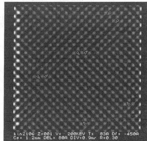
Figure 5: High resolution simulated image generated using the NCEMSS program and a three dimensional extrapolation of the basal plane configuration depicted in Figure 3 as input. The important feature to notice is the development of dark contrast fringes in the 'b' direction of each microdomain. These dark fringes give rise to the "tweed" microstructure seen in Figure 2b. The image is rotated 45 degrees with respect to Figure 4 and the higher intensity spots on the edge of the image are an artifact of the simulation.
