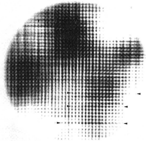
Figure 6b: Processed image of an area extracted from the high resolution image obtained after in-situ beam heating (Figure 2b). Notice the development of orthogonal dark fringes similar to those seen in the simulated image (Figure 5) reflecting the formation of conflicting microdomains in the quenched specimen.
