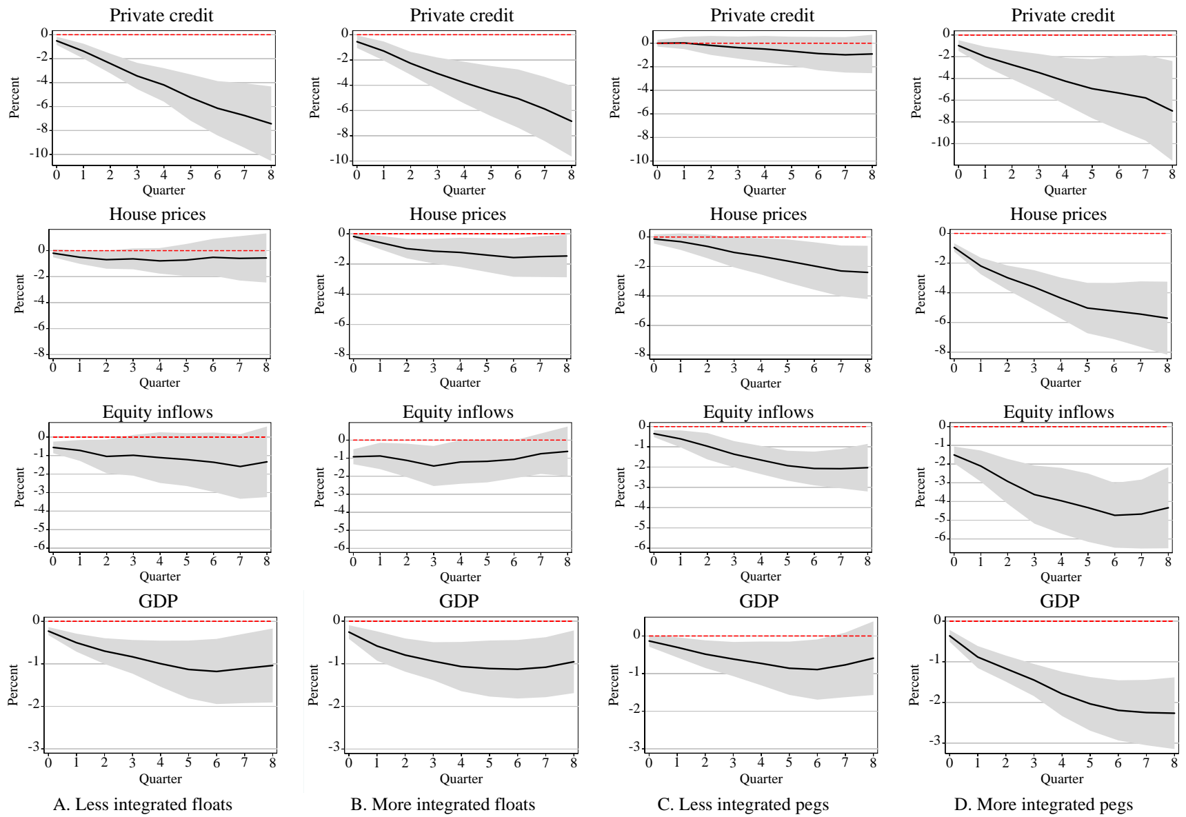
Fig. 2. Cumulative effects of a one-S.D. increase in the VIX.
