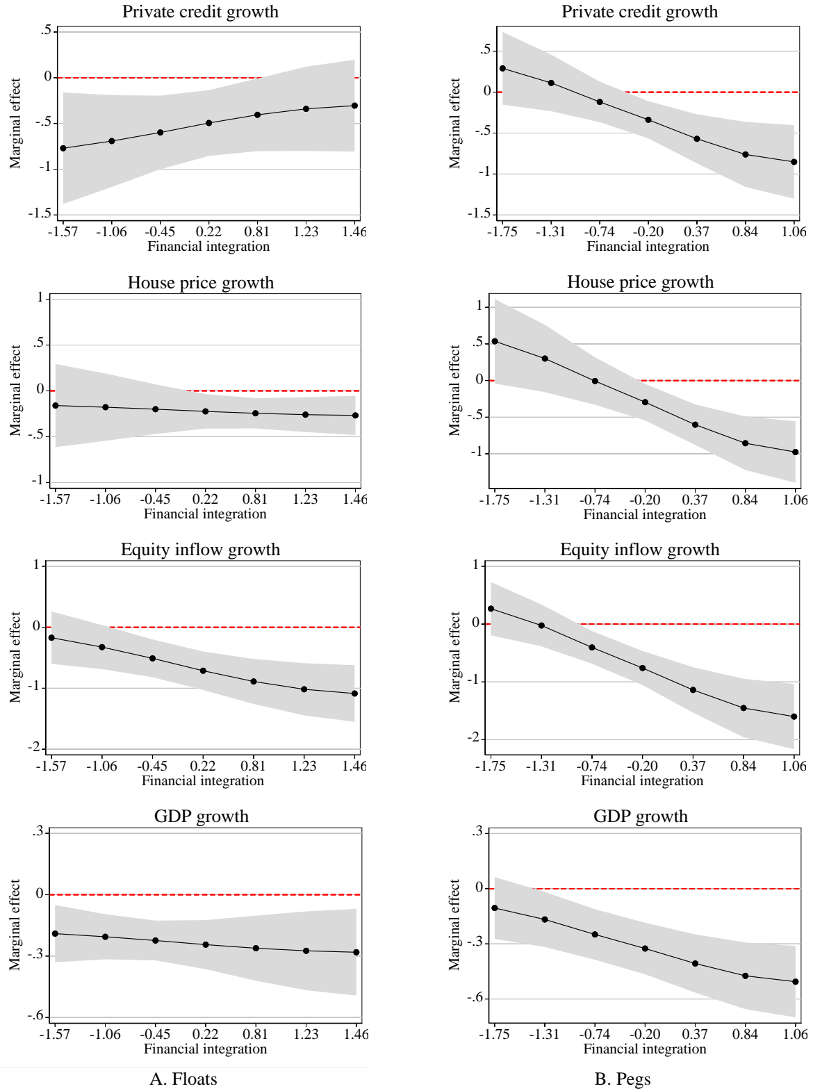
Fig. 1. Marginal effects of the VIX as a function of financial integration. The reported integration values correspond to their subsample distribution at the 5 th , 10 th , 25 th , 50 th , 75 th , 90 th , and 95 th percentiles.
