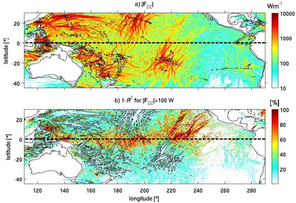
Figure 1: (a) The magnitude of the semidiurnal band-passed energy fluxes in the equatorial Pacific from HYCOM for the month of September 2012. In this month the flux incoherence near the equator is strong (Fig. 3a). Bathymetry is contoured at 0 and -2000 m. (b) The ratio of the sum of the incoherent and cross-term fluxes to the band-passed fluxes. Values coinciding with |\mathbf{F}_{D2}| < 100 \text{ W m}^{-1} are not shown. The black contours mark 1000 \text{ W m}^{-1} of the band-passed fluxes. The equator is marked by the dashed black line.
