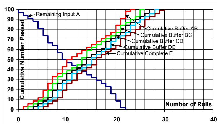
Figure 2. Output from single iteration simulation where all players have die A (All-5)
