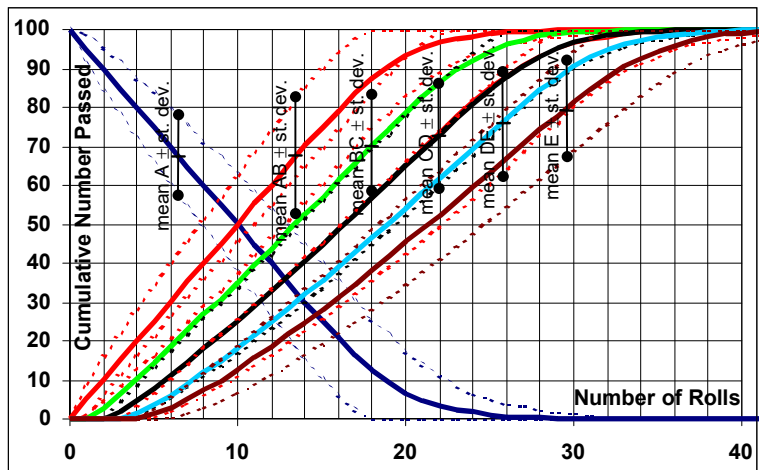
Figure 7. Output from 1,000 iteration simulation where all players have die E (1-9)
