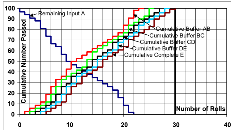
Figure 3. Output from single iteration simulation where all players have die C (3-7)
