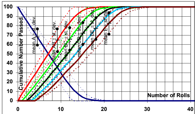
Figure 8. Output from 1,000 iteration simulation where all players have fast die (3-11)
