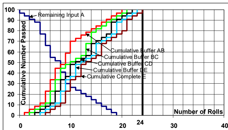
Figure 5. Output from single iteration simulation where all players have die with increased average roll of 7 (3-11)
