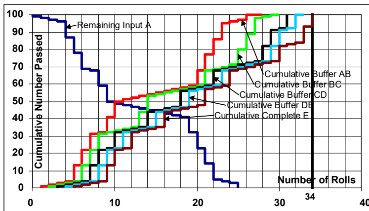
Figure 4. Output from single iteration simulation where all players have die E (1-9)
