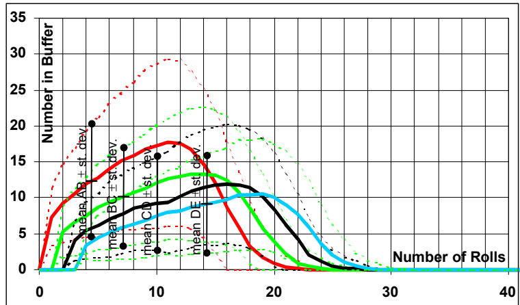
Figure 11. Buffer size from 1,000 iteration simulation where all players have fast die (3-11)
