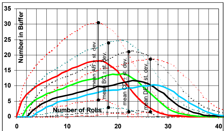
Figure 10. Buffer size from 1,000 iteration simulation where all players have die E (1-9)
