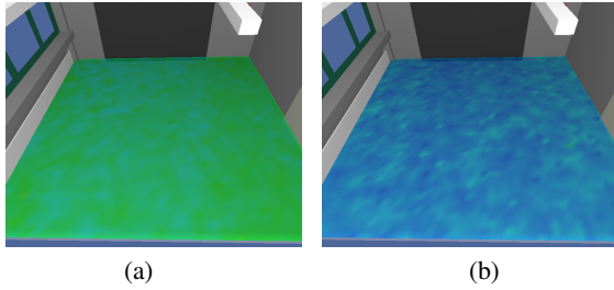
Figure 5: Energy on the floor after the 5th (a) and 10th (c) reflection for the 2560Hz band.
