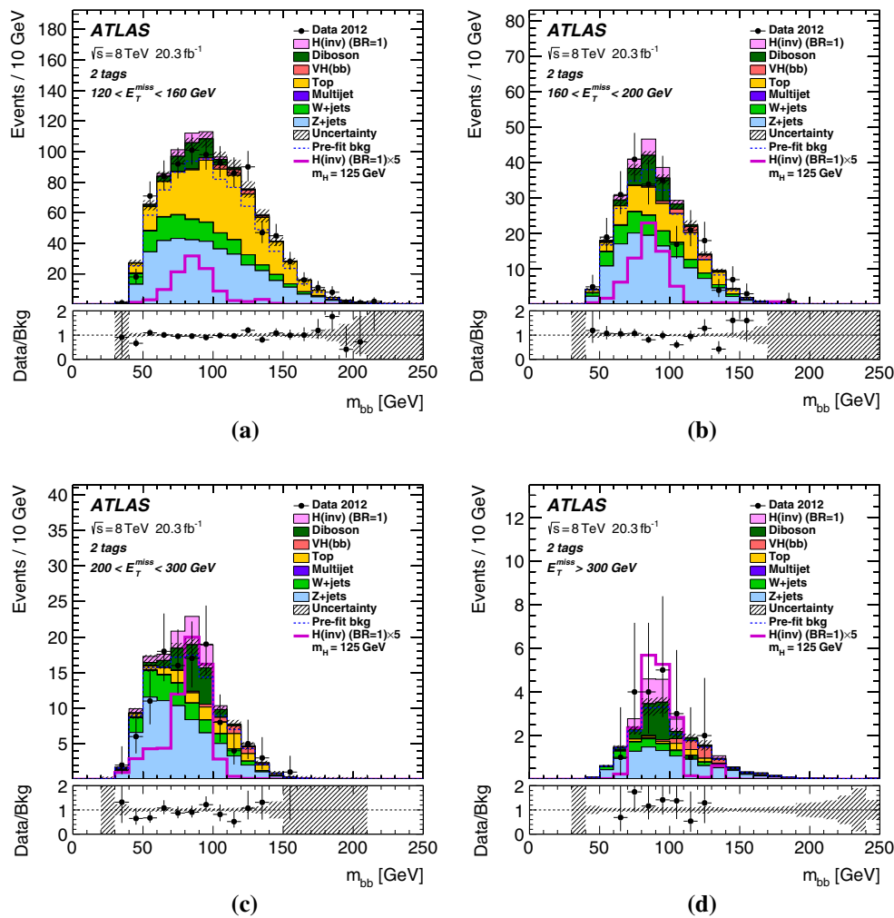
Fig. 5 The dijet invariant mass ( m_{bb} ) distributions in the signal region for the 2- b -tag category, for events with E_T^{miss} in the range a (120–160 GeV), b (160–200 GeV), c (200–300 GeV) and d (>300 GeV). The data are compared with the background model after the likelihood fit. The bottom plots show the ratio of the data to the total background.
