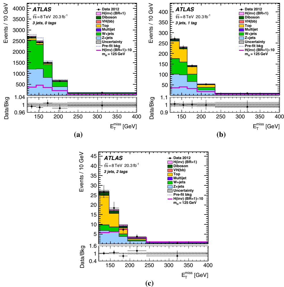
Fig. 2 The missing transverse momentum ( E_T^{\text{miss}} ) distributions of the 3-jet events in the signal region for the a 0- b -tag, b 1- b -tag and c 2- b -tag categories. The data are compared with the background model after the likelihood fit. The bottom plots show the ratio of the data to the total background. The signal expectation for m_H = 125 \text{ GeV} is shown on top
