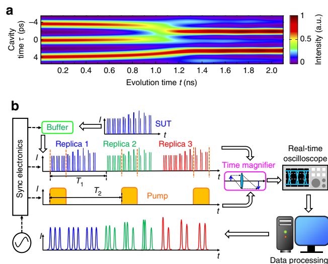
Fig. 1 Working principle of the PARTI system. a Slowly evolved dissipative Kerr soliton dynamics in an ultrahigh- Q microresonator, obtained by numerically solving the Lugiato-Lefever equation. The orders-of-magnitude difference in the timescale between the cavity time and the evolution time poses an experimental challenge to capture the comprehensive picture of the dynamics. b The schematic representation of the PARTI system. The optical buffer generates multiple replicas (represented by blue, green and red, respectively) of the SUT waveform and the subsequent time magnifier captures different portions of the SUT waveform on each replica. After data processing on the system output, the original long SUT waveform can be reconstructed through waveform stitching
