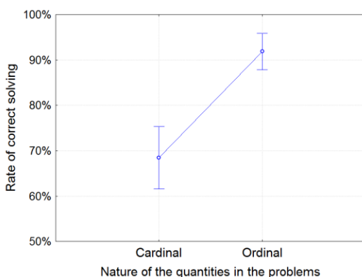
Figure 3: Rate of correct solving on solvable problems. Vertical bars denote 0.95 confidence intervals.
