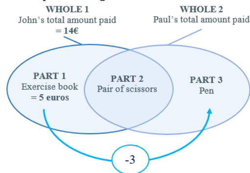
Figure 1.a: Cardinal representation of headcount problems such as those found in Gamo, Sander & Richard (2010).
