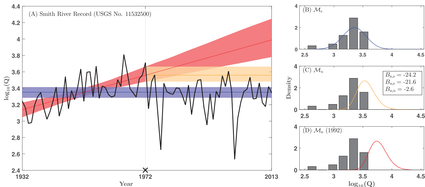
Figure 8. (a) The MAP estimate of the LPIII mean under \mathcal{M}_s (blue line), \mathcal{M}_u (gold line), and \mathcal{M}_n (red line) shown over the full record length (black line). The colored shading represents the respective 95% credible intervals of the the LPIII mean. (b–d) Predictions of out-of-sample density under \mathcal{M}_s (blue line), \mathcal{M}_u (gold line), and \mathcal{M}_n (red line) derived from the MAP parameter estimate. The black histograms show the empirical density in the evaluation period. For the Smith River record, \mathcal{M}_s most accurately predicted the out-of-sample data, which is reflected by B_{n,s} and B_{u,s} shown in Figure 8c.
