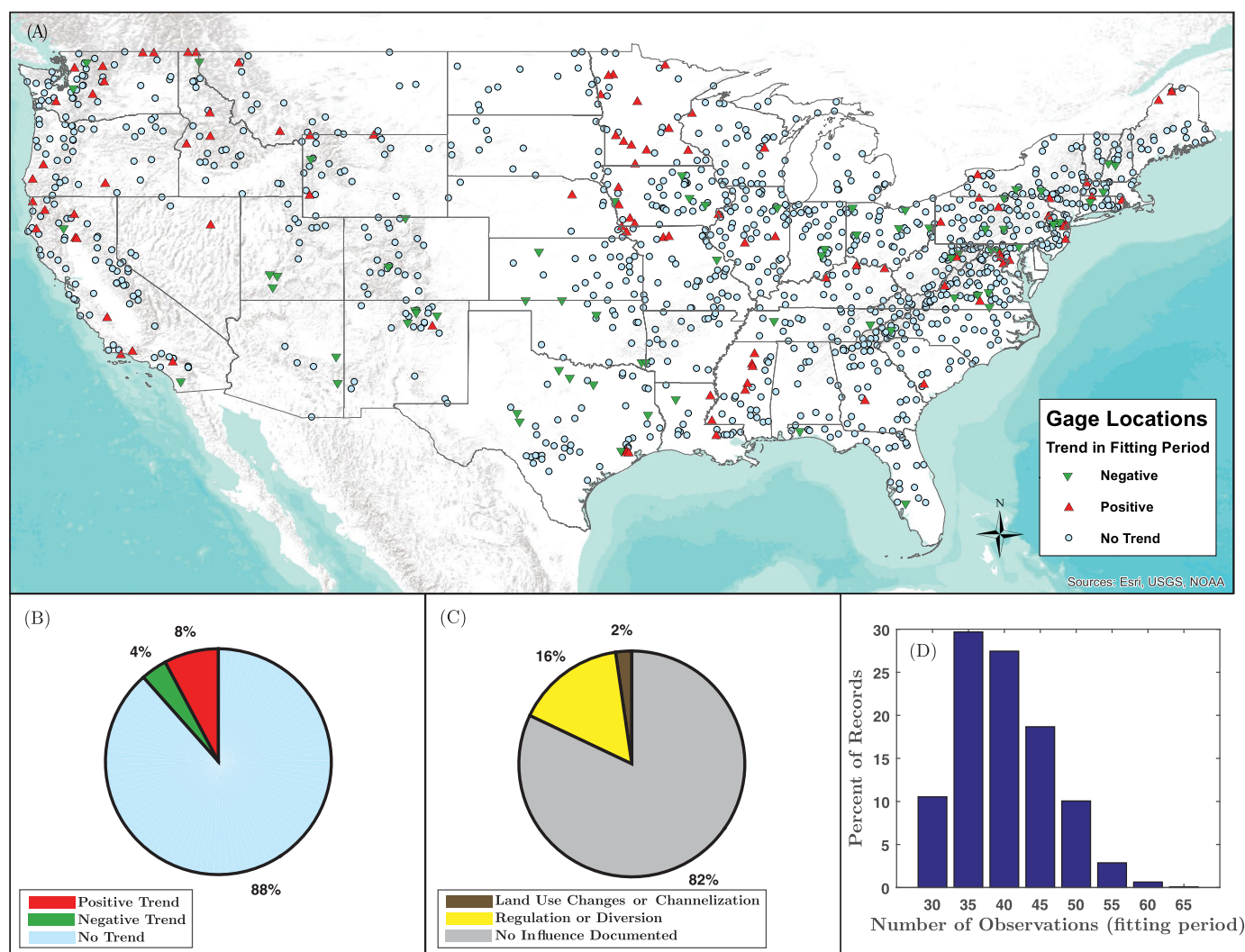
Figure 3. (a) Location of annual maximum discharge records and trends detected according to the Mann-Kendall trend test at the 0.05 significance level. (b) Fitting period trend characteristics as a percentage of all records tested. (c) Anthropogenic watershed influences as a percentage of all records tested. Land use changes or channelization refers to USGS record flag “C,” while regulation and diversion refers to USGS record flag 5 or 6. (d) Fitting period length as a percentage of all records tested.
