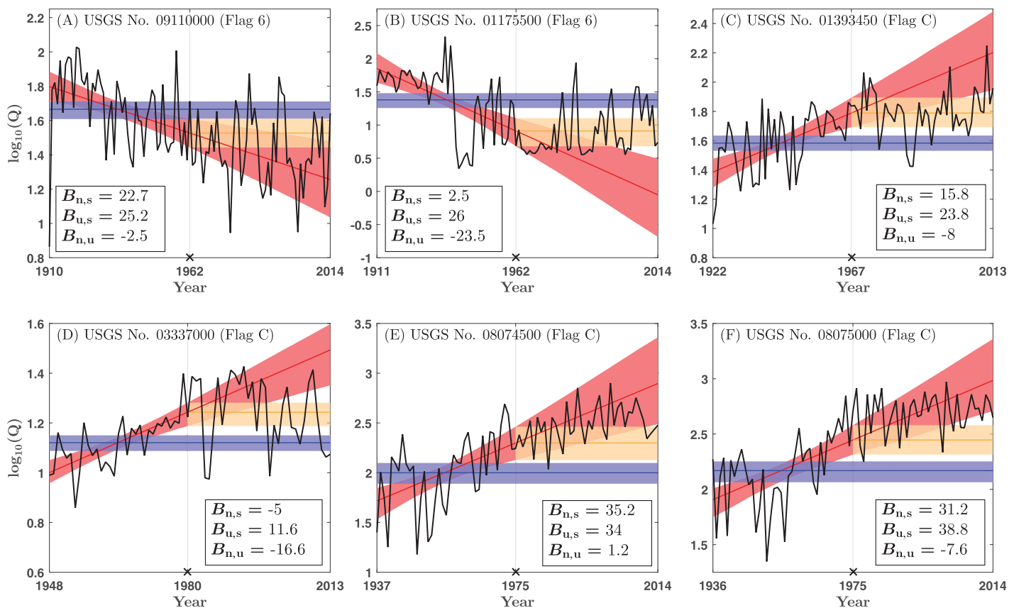
Figure 12. The MAP estimate of the LPIII mean under \mathcal{M}_s (blue line), \mathcal{M}_u (gold line), and \mathcal{M}_n (red line) shown over the full data record (black line). The colored shading represents the respective 90% credible intervals of the LPIII mean, and the black cross denotes the end of the fitting period. The Bayes factor values are shown in the text boxes. Records (a–f) belong to category (b) of Figure 10, i.e., they exhibit a significant trend in the fitting period and discharges are affected by land use changes or channelization (flag C), upstream regulation, or diversion (flag 6).
