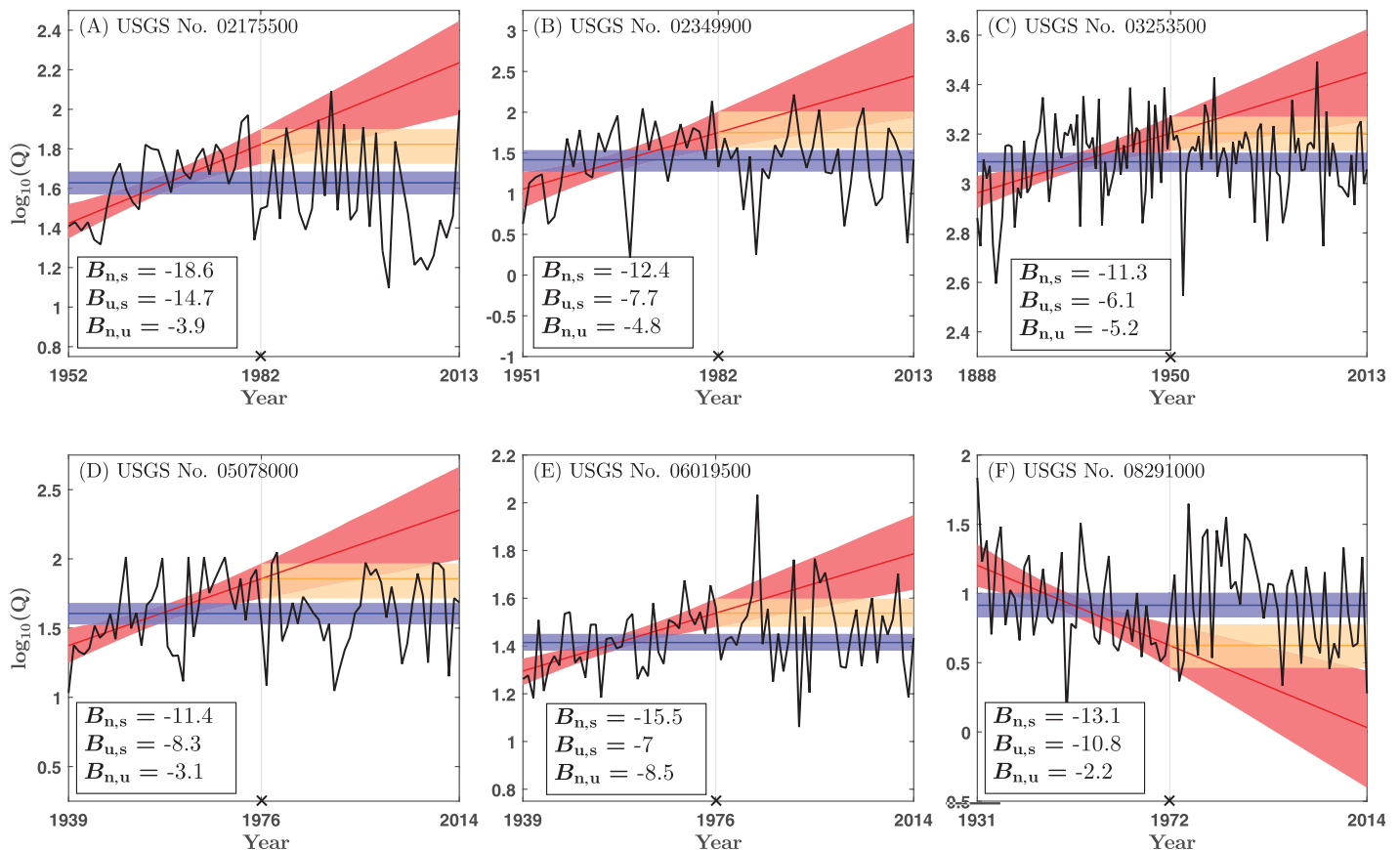
Figure 11. The MAP estimate of the LPIII mean under \mathcal{M}_s (blue line), \mathcal{M}_u (gold line), and \mathcal{M}_n (red line) shown over the full data record (black line). The colored shading represents the respective 90% credible intervals of the LPIII mean, and the black cross denotes the end of the fitting period. The Bayes factor values are shown in the text boxes. Records (a–f) belong to category (a) of Figure 10, i.e., they exhibit a significant trend in the fitting period and DIC favors the NS model.
