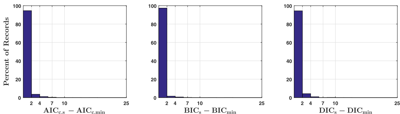
Figure 6. Comparison of model fit between the ST and NS models. (row a) Displays the differences in metric values for fitting periods with a detected trend (145 total) and (row b) displays the differences for fitting periods without detected trends (1105 total). Each column represents a different goodness of fit metric. The magnitude of the differences represents the level of empirical support for the ST model. Values from 0 to 2 in each figure indicate substantial support, values from 4 to 7 indicate considerably less, and values greater than 10 indicate essentially no empirical support for the ST model [Burnham and Anderson, 2003]. These results demonstrate that the presence of a trend substantially reduces the level of empirical support for the ST model relative to the NS model.
