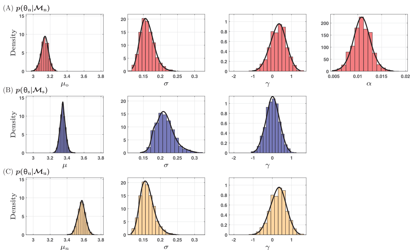
Figure 7. Prior parameter density for the evaluation period (black lines) under (row a) \mathcal{M}_n , (row b) \mathcal{M}_s , and (row c) \mathcal{M}_u defined by the GMM fit to the posterior distributions of the Smith River fitting period (red, blue, and gold histograms). The additional complexity under \mathcal{M}_n is accounted for through its four dimensional prior. Increased parameter uncertainty of \mu_n is represented by its lower and more dispersed prior density relative to \mu .
