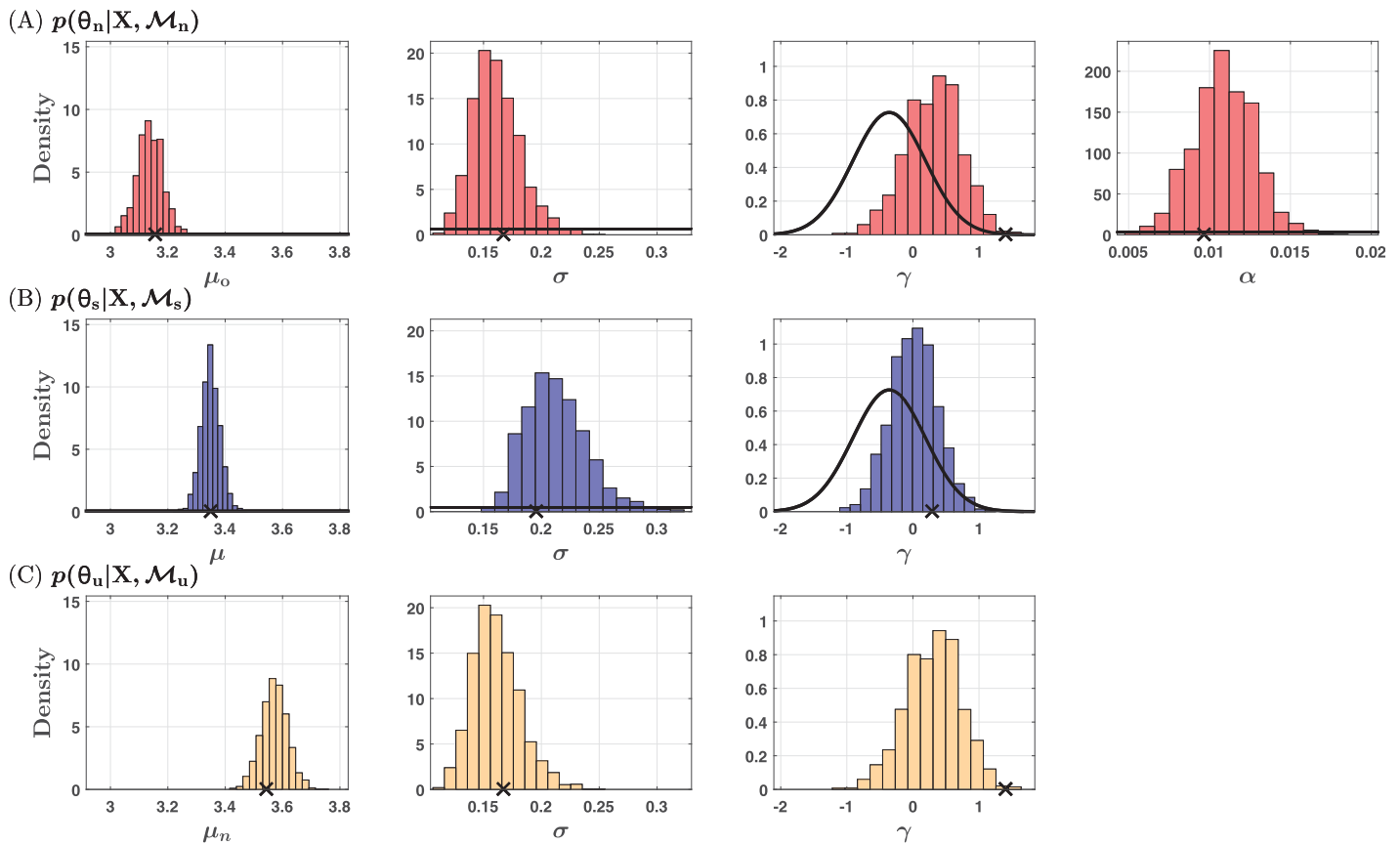
Figure 4. Marginal posterior distributions of \theta_n under the NS model (red histograms), \theta_s under the ST model (blue histograms), and \theta_u under the uST model (gold histograms), given the data in the Smith River fitting period. Black lines represent the marginal prior distributions, and the black crosses show the MLE of \theta_j under the three models. Notice that the MLE of \gamma under \mathcal{M}_n is very unlikely according to the prior distribution, and posterior \theta_n favors lower values of \sigma than posterior \theta_s .
