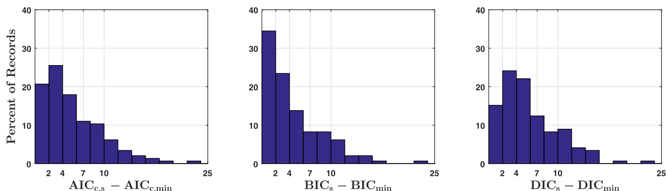
(B) No trend detected in fitting period
