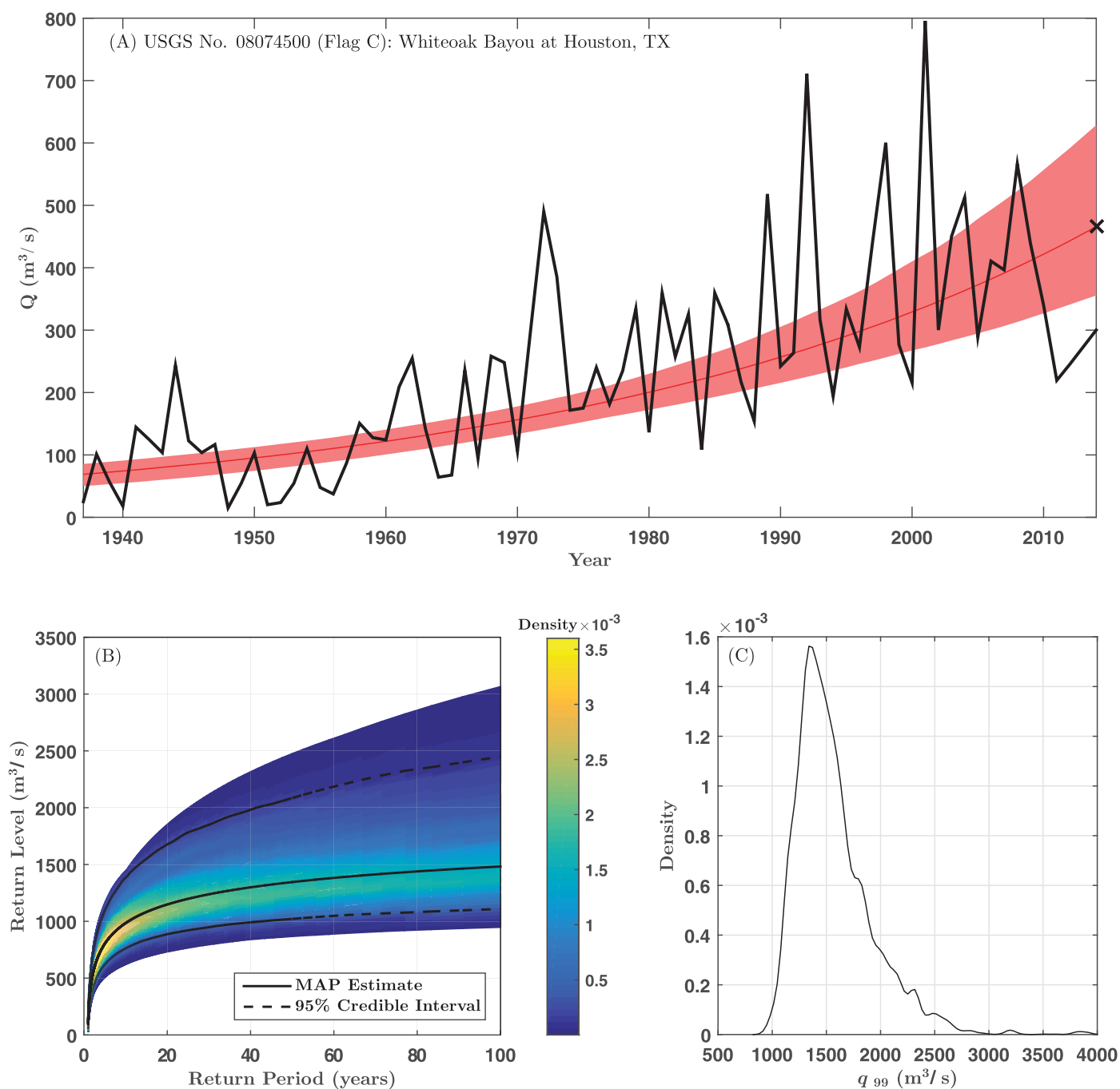
Figure 13. (a) The MAP estimate of the NS LPIII mean and 95% credible interval (red line and shading) inferred from the full record length (black line), shown outside of the log-space. The black cross denotes the mean of the uST distribution. (b) Return level versus return period plot derived from the uST distribution. The solid black line represents the MAP estimate of each return level, and the dashed black lines represent the 95% credible interval. The density of the return level estimates is shown on the color bar, which are readily available from the posterior sample of \theta_u . (c) Distribution of the q_{99} estimates (or 100 year return level) under the uST model.
