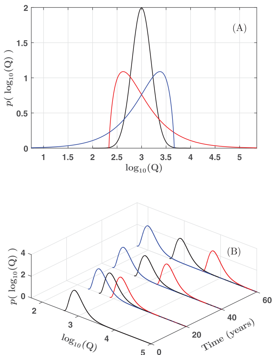
Figure 1. (A) ST LPIII distribution with variable shape parameter. The red, black, and blue lines correspond to \gamma values of 1.5, 0, and -1.5 , respectively. (B) NS LPIII distribution with variable trend parameter. The red, black, and blue lines correspond to \alpha values of 0.015, 0, and -0.015 , respectively.
