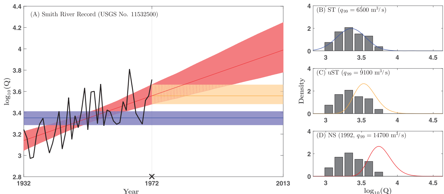
Figure 2. (a) Maximum a posteriori (MAP) estimate of the LPlll mean under the ST (blue line), uST (gold line), and NS (red line) models inferred from the Smith River fitting period Q (black line). The colored shading represents the respective 95% credible intervals of the LPlll mean, and the black cross denotes the end of the fitting period. (b–d) Predictions of out-of-sample density under the ST (blue line), uST (gold line), and NS (red line) models derived from the MAP parameter estimates. The black histograms represent the empirical density of the fitting period. Notice that Figures 2c and 2d show predictions under the uST and NS models moving away from the observed density, and the 95% credible intervals are wider under the NS and uST models relative to the ST model.
