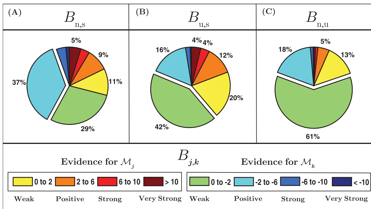
Figure 9. Bayes factor value as a percentage of all records tested (1250 total). (a) Bayes factor for \mathcal{M}_n and against \mathcal{M}_s . (b) Bayes factor for \mathcal{M}_u and against \mathcal{M}_s . (c) Bayes factor for \mathcal{M}_n and against \mathcal{M}_u . Yellow to red values support \mathcal{M}_j , which is \mathcal{M}_n in Figures 9a and 9c, and \mathcal{M}_u in Figure 9b. Green to blue colors support \mathcal{M}_k , which is \mathcal{M}_s in Figures 9a and 9b and \mathcal{M}_u in Figure 9c. Results in Figure 9a show that the evidence supports predictions under \mathcal{M}_s relative to \mathcal{M}_n for about 70% of records tested, with 40% of records exhibiting at least positive evidence for \mathcal{M}_s . Results in Figure 9b show that predictions under \mathcal{M}_s are also preferred relative to \mathcal{M}_u , except here the majority of evidence only weakly supports \mathcal{M}_s . Interpretation of the Bayes factor values is based on Kass and Raftery [1995].
