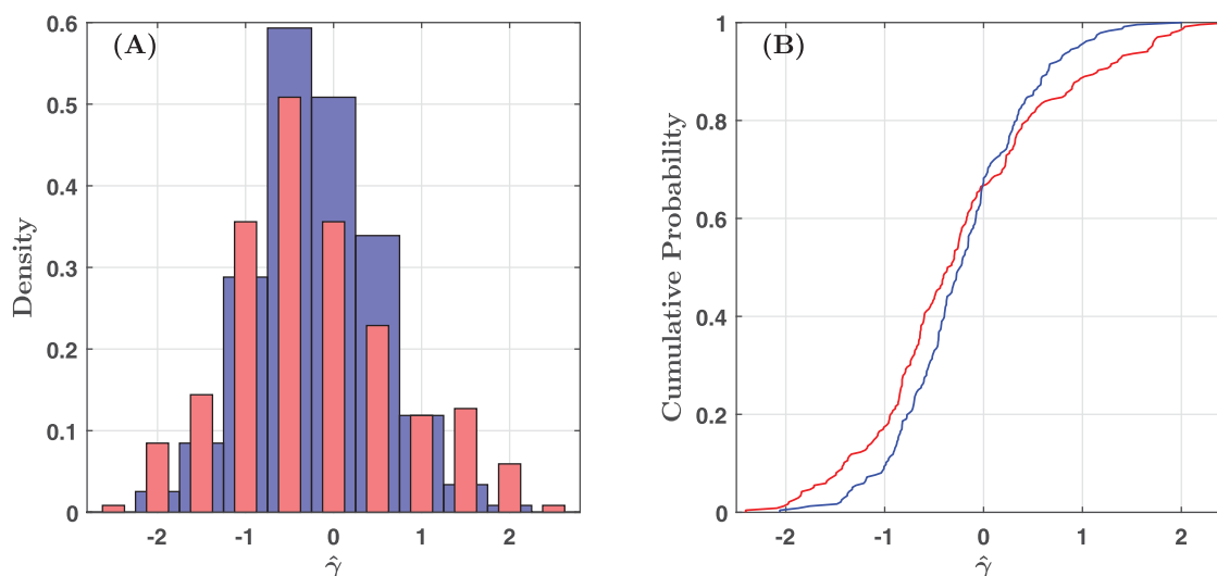
Figure 5. (a) Empirical density of \hat{\gamma} under the NS model (red histogram) and the ST model (blue histogram) based on the estimates from fitting periods where \hat{\alpha} was one standard deviation away from the mean of zero (236 total). The circumflex denotes the MLE of \gamma and \alpha . (b) Empirical CDF of \hat{\gamma} under the NS model (red line) and ST model (blue line). The CDF of \hat{\gamma} under the NS model is different from the ST model counterpart, indicating that the likelihood function favors larger values of \hat{\gamma} (i.e., \pm 1.4 ) under the NS model. Indeed, there is a difference between the two CDFs at the 0.05 significance level according to the two sample Kolmogorov-Smirnov test [Massey, 1951].
