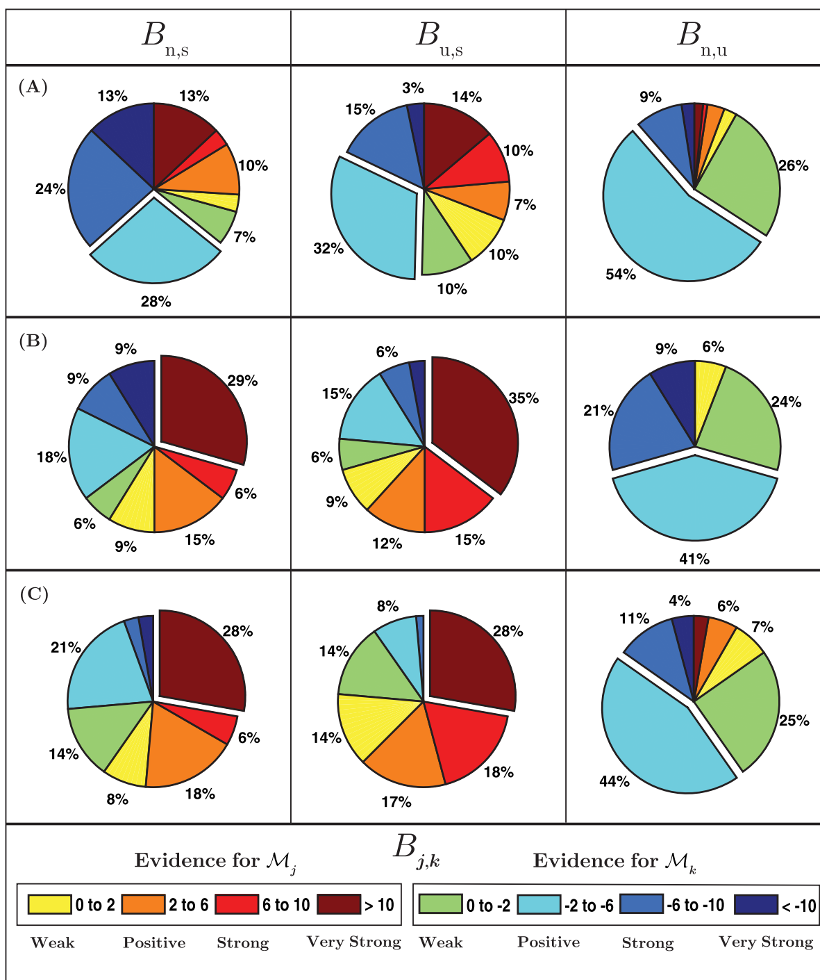
Figure 10. Bayes factor value as a percentage of records with detected trends in the fitting period and (a) DIC significantly favoring \mathcal{M}_n (123 total), (b) discharges affected by land use changes, regulation, or diversion (34 total), and (c) trend also detected using full record length (72 total). The columns compare the evidence between competing models in the same manner as Figure 9. (a) Reveals that the presence of a trend and DIC favoring the NS model does not improve the relative success of \mathcal{M}_n compared to all records tested in Figure 9. (b) Shows that \mathcal{M}_u is strongly preferred for prediction relative to \mathcal{M}_s and \mathcal{M}_n if a trend is accompanied by physical watershed changes.
