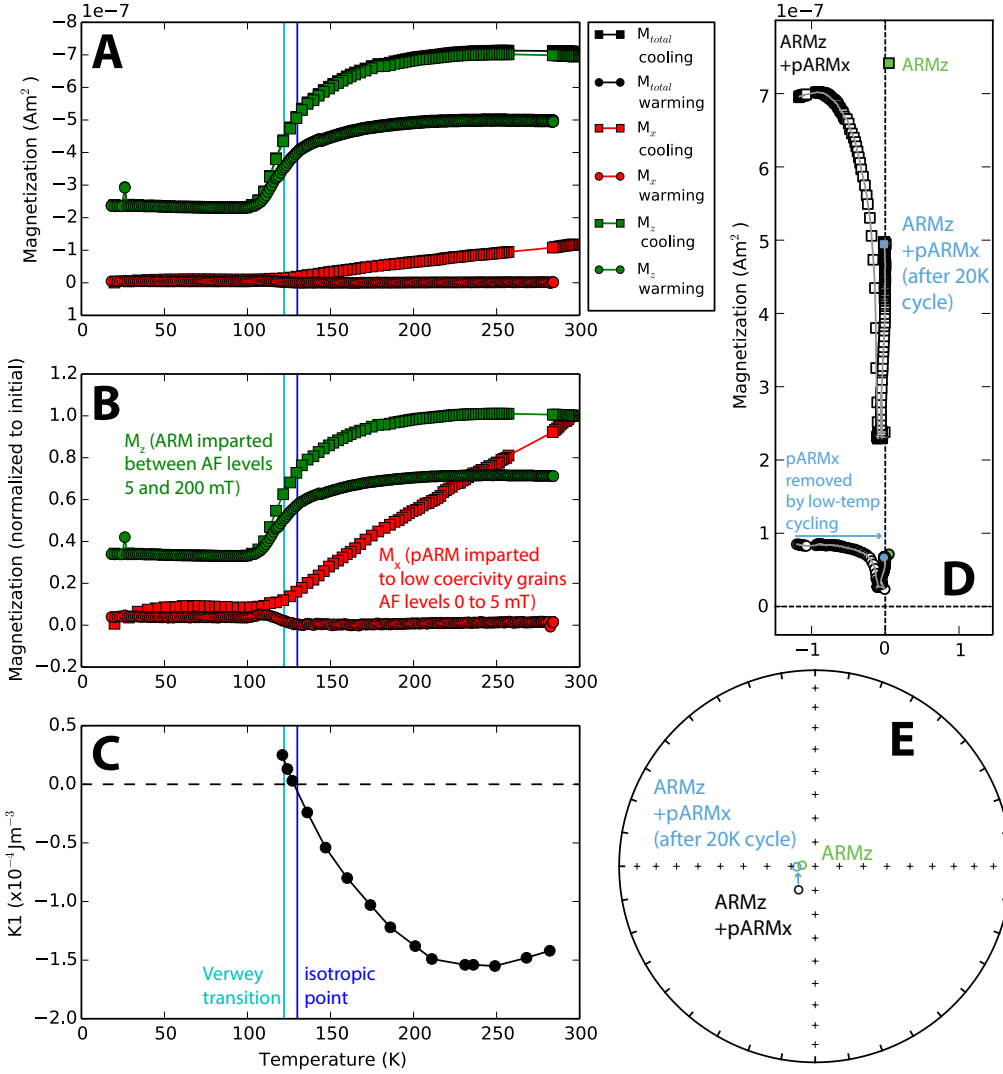
Figure 8. Low-temperature behavior of an ARM applied to the z-axis and a pARM applied to the x-axis of a specimen of an Umkondo diabase sill (PW15-4d). (a) shows the magnetization of the z and x components as well as the total magnetization upon cooling (note that the y-axis of the plot is inverted for comparison between the components and the total magnetization). The z and x components are normalized to their initial magnetizations in (b) to highlight the differing behavior between the x-axis magnetization (pARM imparted to low coercivity grains) and the z-axis magnetization (ARM on the rest of the coercivity spectrum). (c) shows the magnetocrystalline anisotropy constant K_1 as a function of temperature (data of Bickford et al. [1957] as presented in Muxworthy and McClelland [2000]). The vector-component diagram (d) and equal area plot (e) show the directional change associated with low-temperature cycling and illustrate the return to the direction of the z-axis ARM with the x-axis pARM demagnetized.
