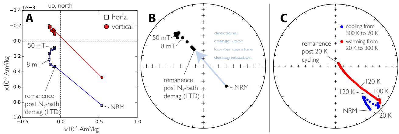
Figure 9. Natural remanent magnetization (NRM) data for a coarse-grained diabase sill sample (PW10-7). (a) Demagnetization data that begins with a low-temperature demagnetization step (a liquid \text{N}_2 bath) followed by AF demagnetization. The vector component diagram in (a) and equal area plot in (b) show significant loss of remanence and directional change that accompanied the liquid \text{N}_2 treatment. (c) Low-temperature cycling of the NRM of a sister specimen on the IRM-LTI documented directional change throughout the experiment with movement in the direction of overprint removal both during cooling to the Verwey transition and upon warming back across the Verwey transition.
