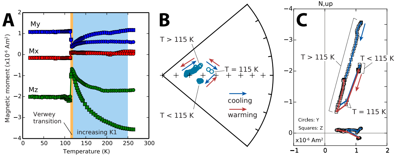
Figure 5. Data from the series 2 experiment (1.2 T IRM applied approximately along the [100] axis) on the single magnetite crystal. (a) three-axis remanence data for cooling to 20 K and warming back to room temperature using the IRM-LTI. The orange box indicates the interval over which the specimen passes through its Verwey transition, while the blue box indicates the interval of remanence loss as the specimen approaches its isotropic point. (b) portion of an equal area plot of the remanence direction during thermal cycling illustrating the clockwise change that occurs as the sample is cooled through the Verwey transition. This directional change is reversible on warming. (c) vector component diagram where both the change in direction and increase in intensity can be seen across the Verwey transition. The blue line connects data points measured during the cooling portion of the experiment while the red line connects data points for the warming portion of the experiment.
