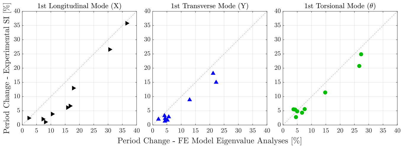
Fig. 7 Percent change in period, compared with virgin state, as estimated using experimental data (SI-based, WN) and numerical data (FE-model-based, eigenvalue analyses)
