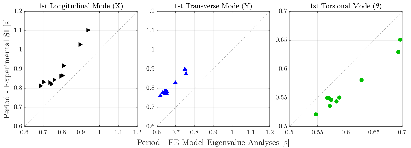
Fig. 6 Period evolution comparison between experimental SI-based and FE-model-based results.
