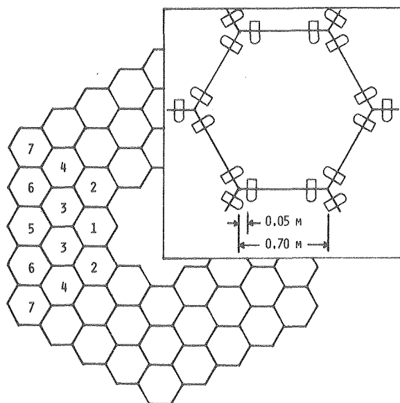
Fig. 2. The primary mirror, with the different mirror types labeled. The inset shows the approximate location of the displacement sensors on a segment
