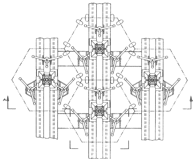
Fig. 18. Top view of support structure
