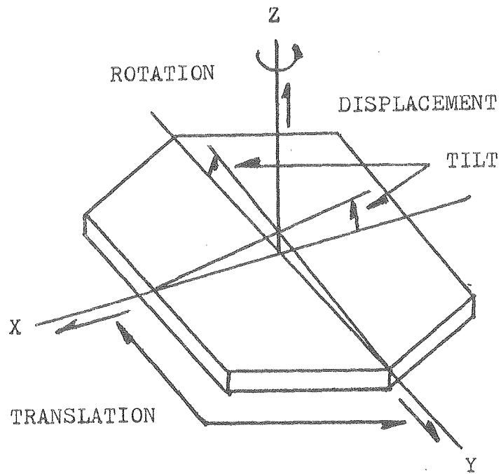
Fig. 3. The six motions of a segment
