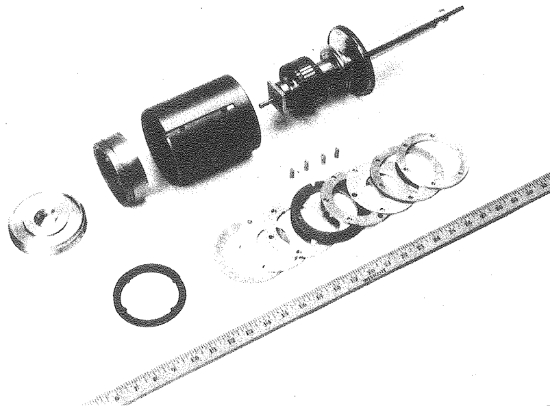
Fig. 14. Partially disassembled inner housing assembly
