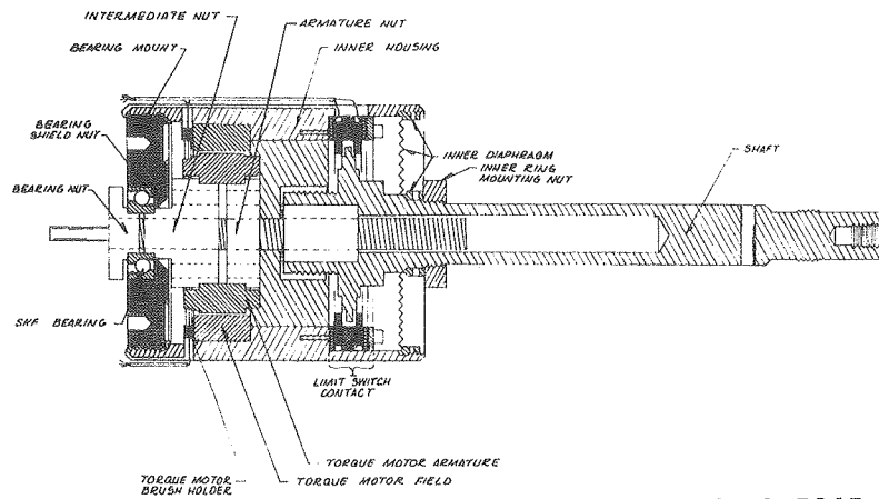
Fig. 13. TMT precision servo actuator inner housing assembly
