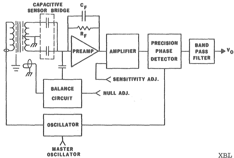
Fig. 5. Block diagram of displacement detector
