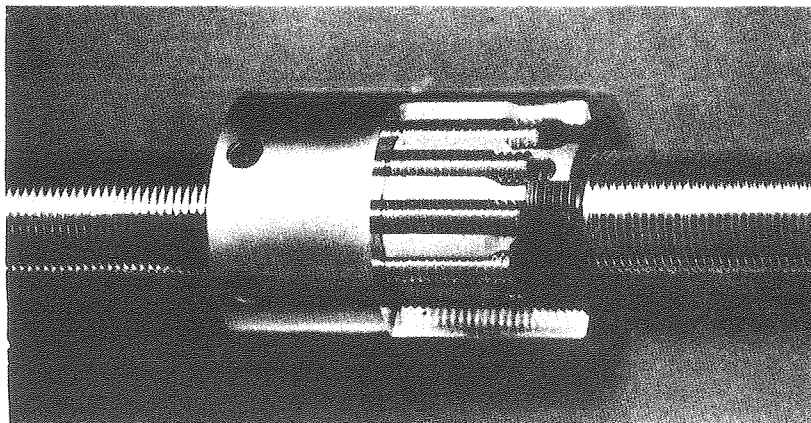
Fig. 10. Planetary roller screw
