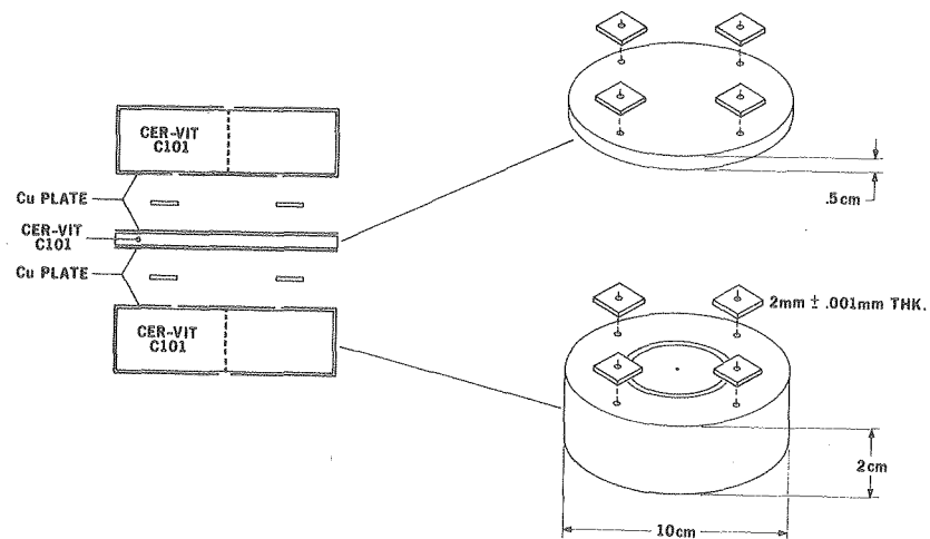
Fig. 6. Mechanical configuration for test displacement sensor
