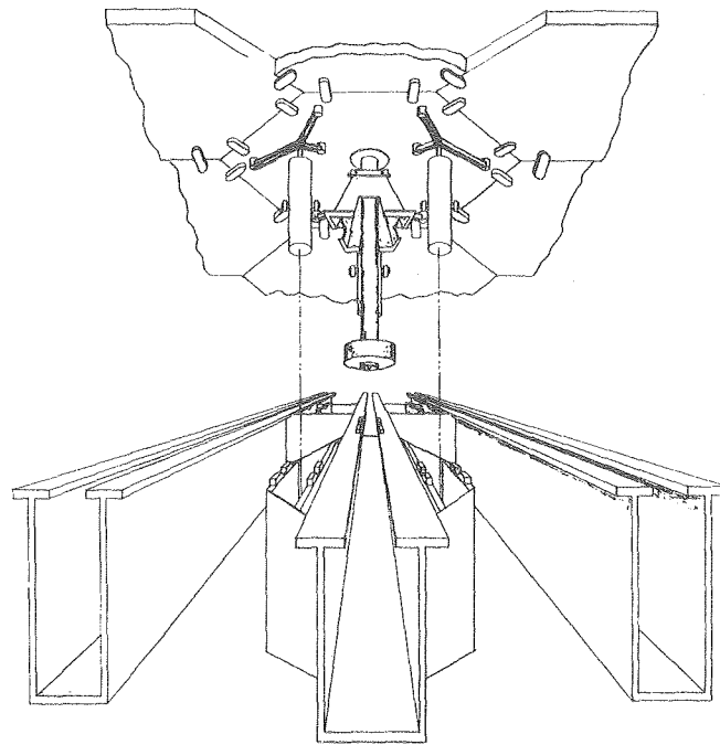
Fig. 19. Perspective of support structure
