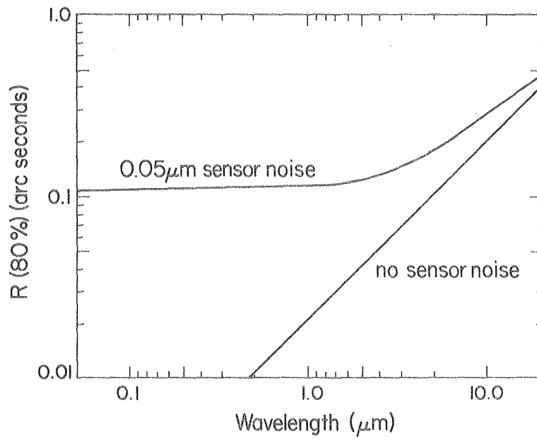
Fig. 4. Effect on image quality versus wavelength for optically perfect segments and two sensor noise levels
