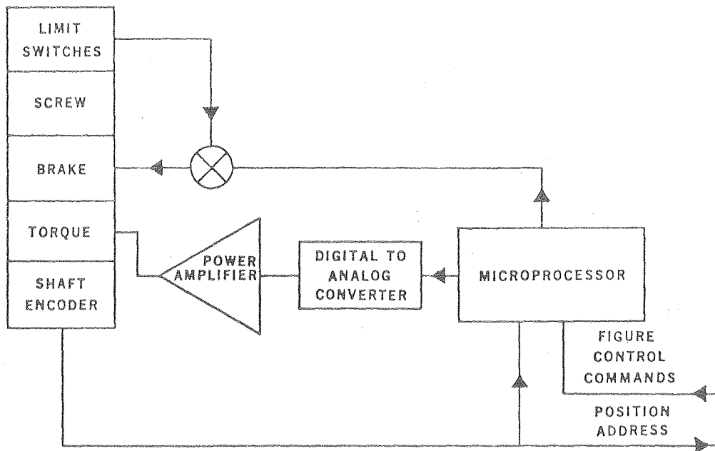
Fig. 12. Block diagram of displacement actuator
