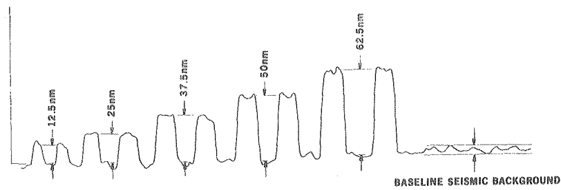
Fig. 11. Roller screw displacement response for incremental step input
