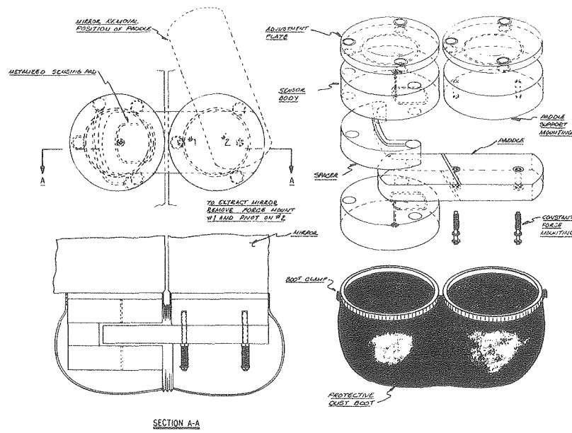
Fig. 9. Displacement sensor
