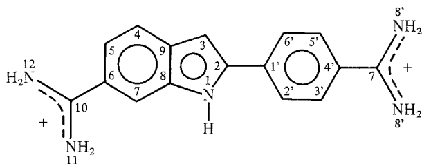
Scheme 1. Structure of 4'-6-diamidino-2-phenylindole (DAPI)
