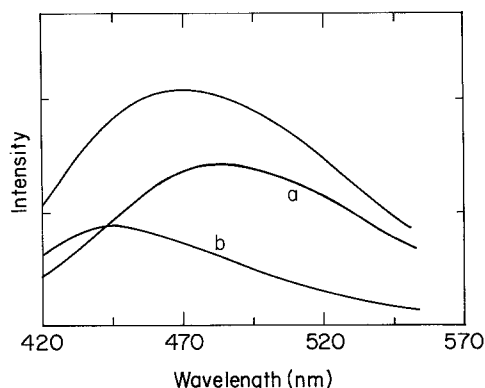
Fig. 5. Phase and modulation resolved spectra of DAPI at pH = 7.1. Excitation at 325 nm; modulation frequency 100 MHz (a) Spectrum at 0.15 ns and (b) at 2.5 ns
