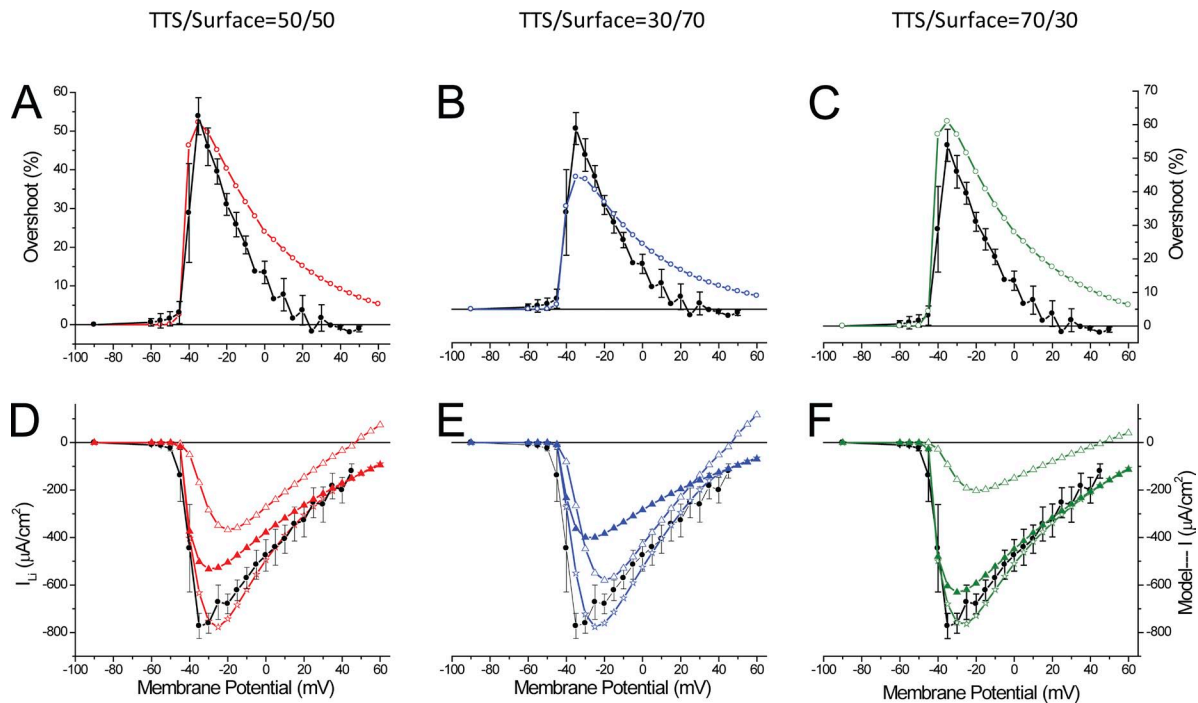
Figure 13. Model predictions of overshoot and currents for various \overline{P}_{Na} distributions in the surface and TTS membranes. (A–C) Voltage-dependent overshoots calculated (see Fig. 11 A) using the following \overline{P}_{Na} -TTS/ \overline{P}_{Na} -S ratios: 1 (or 50:50) in A; 0.429 (or 30:70) in B; and 2.333 (or 70:30) in C. The total values of \overline{P}_{Na} were 12 \times 10^{-4} cm/s, 13.5 \times 10^{-4} , and 11 \times 10^{-4} for the calculations of the overshoot in A, B, and C, respectively. In every panel, the filled black symbols are the average values shown in Fig. 9 A; the superimposed open symbols were obtained with 50:50 (A, red), 70:30 (B, blue), and 30:70 (C, green) S/ \overline{P}_{Na} -TTS, respectively. (D–F) Average peak I-V plots of I_{Li} as shown Fig. 9 B (black symbols) are superimposed with model predictions for 50:50 (A, red symbols), 30:70 (B, blue symbols), and 70:30 (C, green symbols) \overline{P}_{Na} -TTS/ \overline{P}_{Na} -S ratios, respectively. In every panel, open stars represent the total current, filled triangles represent the TTS current component, and open triangles represent the surface membrane current component. The fiber radius used in model simulations was the average for all the experiments (25 \mu m), and R_s was 20 \Omega cm 2 . The rest of the model’s parameters are listed in Tables I and II.
