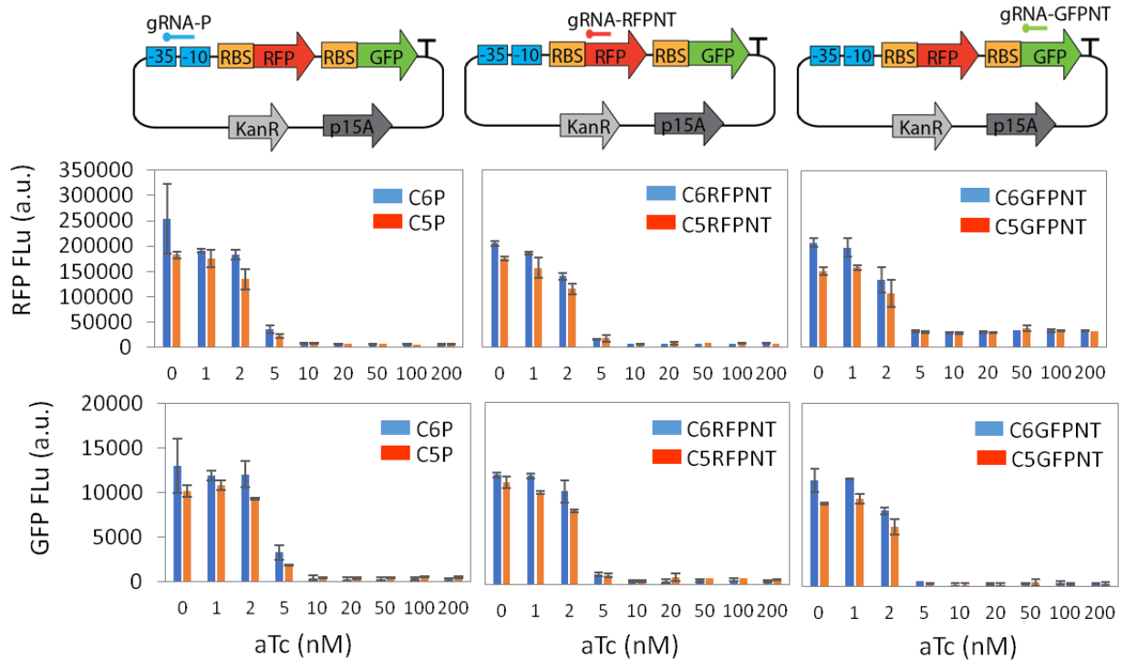
Figure 4 Repression properties of CRISPR-dCas9 system for genes in an operon. Top: Schematics indicating the location of target gRNA in the operon. Middle: RFP fluorescence in response to different gRNA. Bottom: GFP fluorescence in response to different gRNA.
