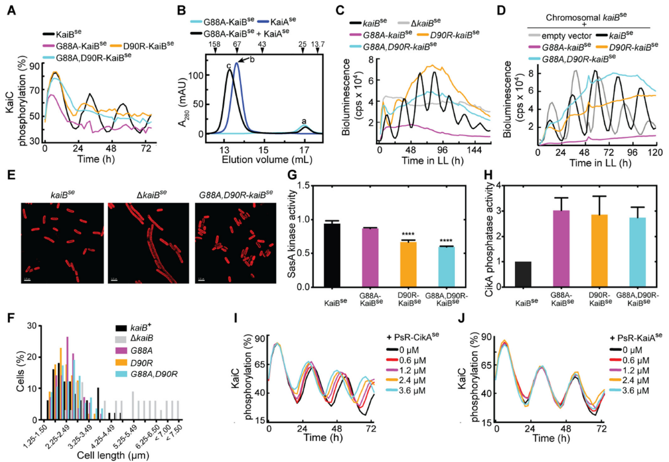
Figure 2. KaiB fold switching regulates oscillator function and clock output
