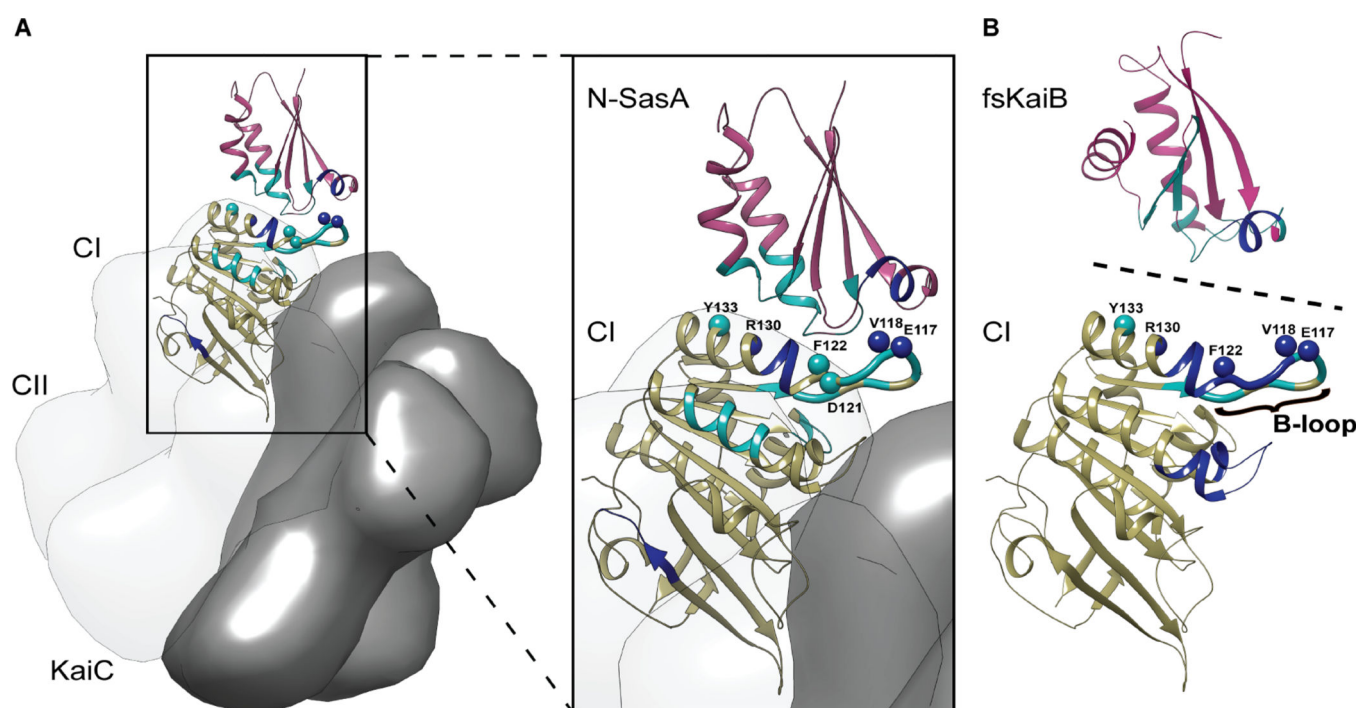
Figure 4. KaiB and SasA bind to similar sites on CI
