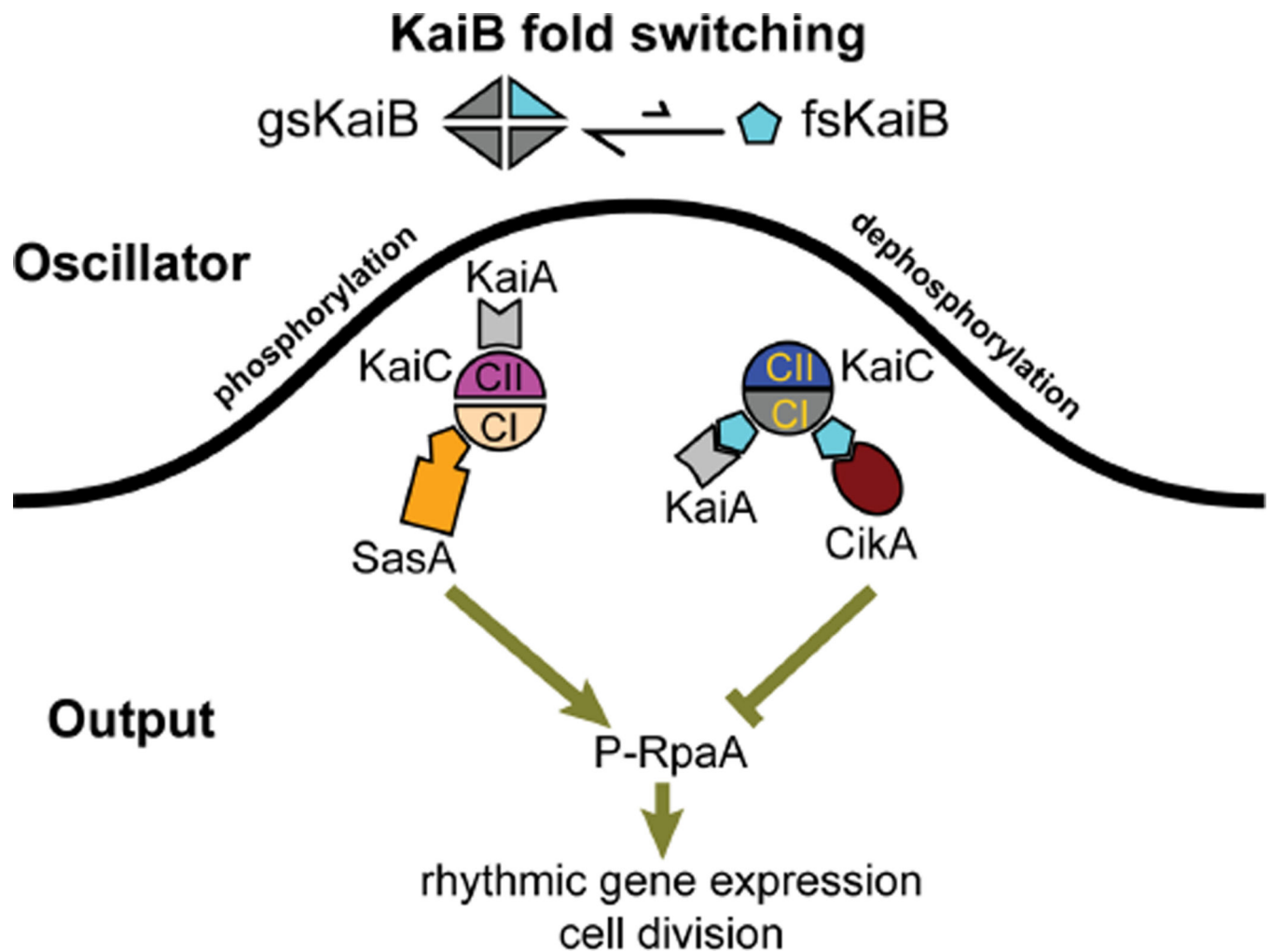
Figure 5. Model of KaiB fold switching as linchpin for the cyanobacterial clock
