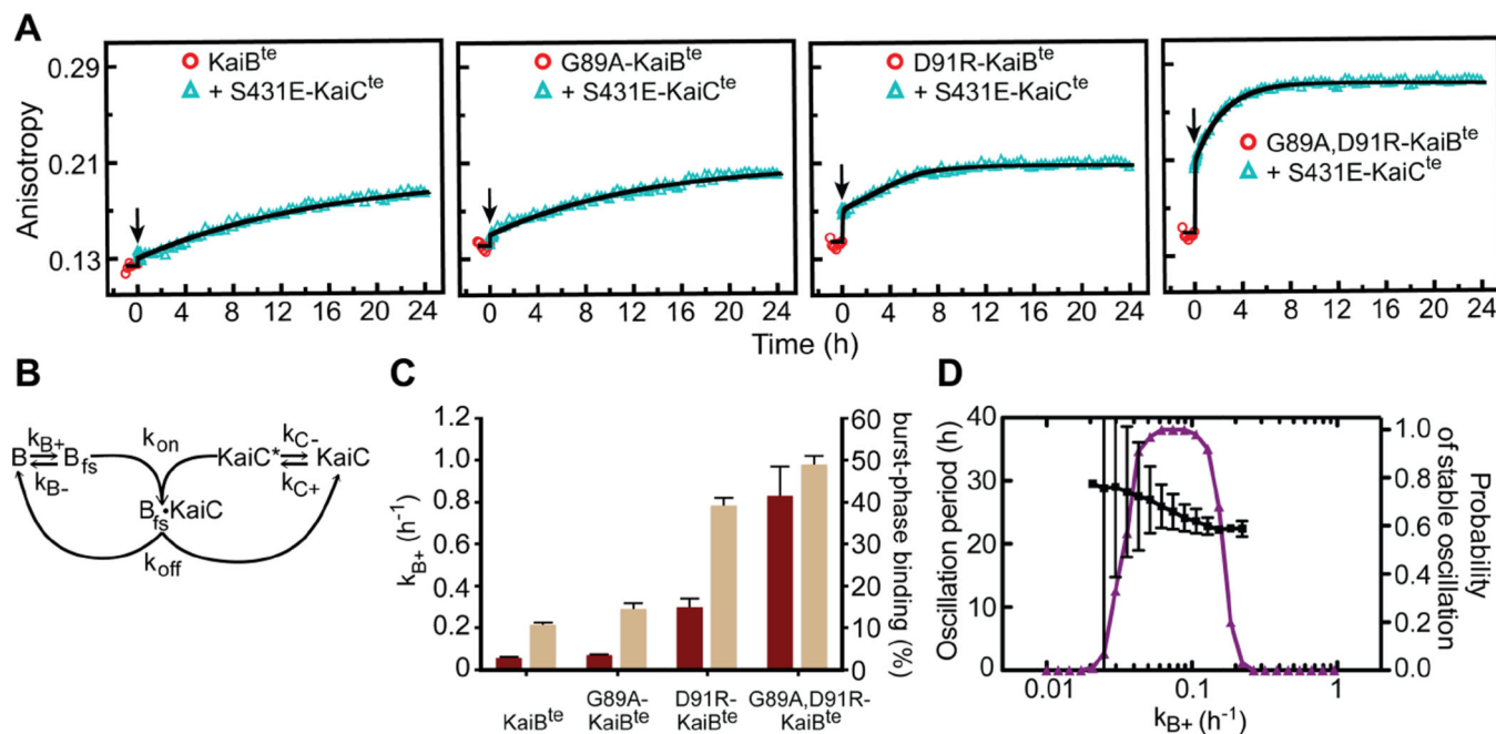
Figure 3. KaiB fold switching regulates slow formation of the KaiB-KaiC complex
