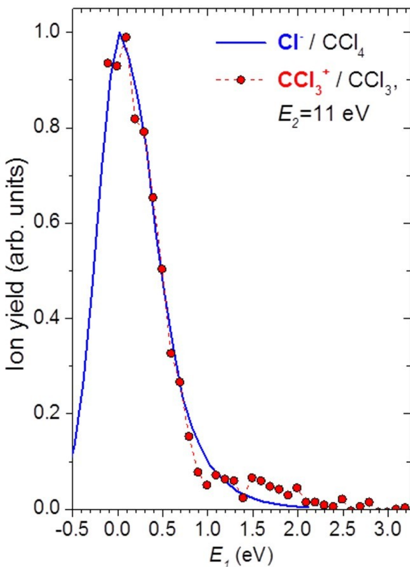
Fig. 11 Ion yield of \text{Cl}^- from the one-step acquisition (blue curve) in which \text{Cl}^- is formed directly from DEA to \text{CCl}_4 and ion yield of \text{CCl}_3^+ from the two-step acquisition, in which in the first step ( E_1 ), \text{CCl}_3 is formed from DEA and in the second step, the neutral \text{CCl}_3 is ionized by electron impact of 11 eV (red circle). Both yields are as a function of the first-step incident electron energy ( E_1 ). Two steps E_1 and E_2 correspond to steps in the experimental procedure presented in Fig. 13(c). Reprinted with permission from [109]. Copyright (2017) by the American Physical Society.
