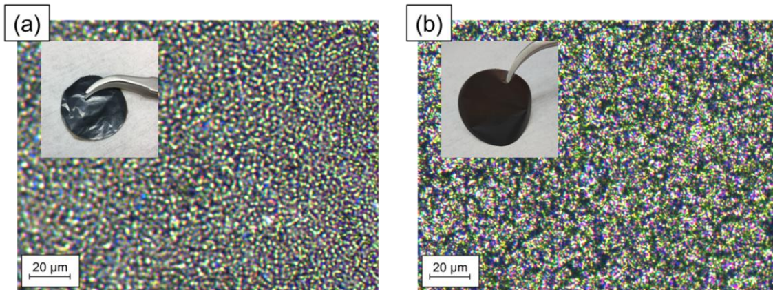
Figure 4.7 (a) the microscope image of GO film fabricated with the help of silicon wafer. The inset depicts photographic image of the respective film. (b) the microscope image of GO film fabricated without the help of silicon wafer. The inset depicts a photographic image of the fabricated film.
