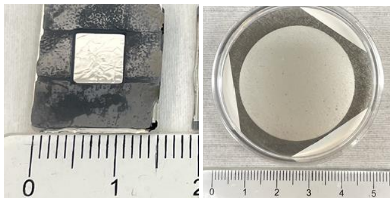
Figure 4.15 The reflective surface is optically smooth when fabricated following the method developed in this study (left), whereas the surface finish of the aluminum deposition is visibly rough when directly applied on top of vacuum filtration CNT films without any further treatment (right).
