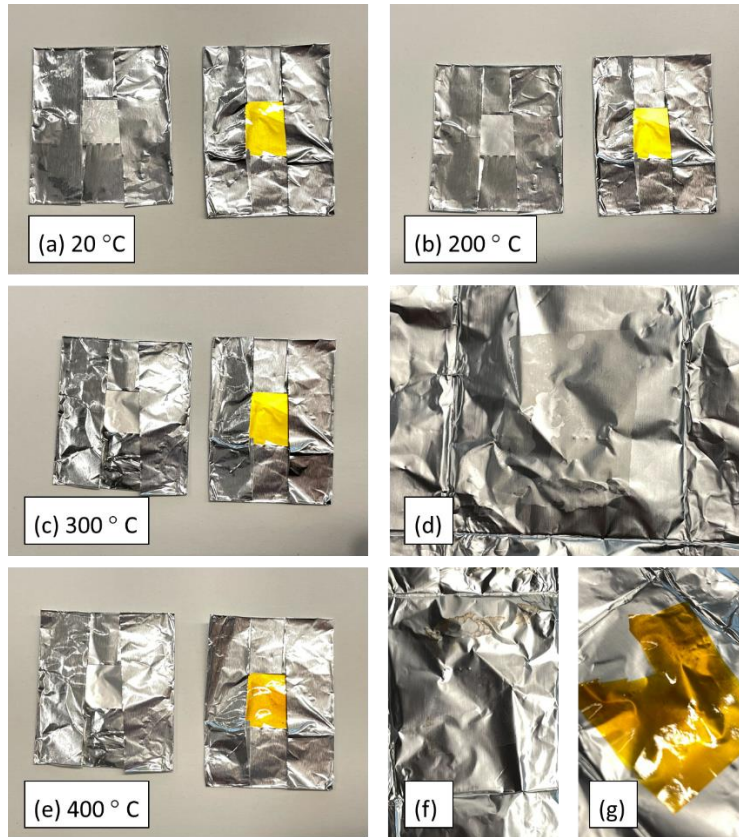
Figure 4.2 (a) 0.5 \mu\text{m} Mylar and 7 \mu\text{m} Kapton film at room temperature (b) after 10 minutes on 200 \text{ }^\circ\text{C} hotplate. (c) after 10 minutes at 300 \text{ }^\circ\text{C} (d) Mylar film damaged at 300 \text{ }^\circ\text{C} (e) after 10 minutes at 400 \text{ }^\circ\text{C} (f) Mylar film mostly gone. (g) Kapton film showing signs of burning.
