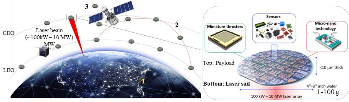
Figure 2.4 Concept of laser propelled wafer scale femtosatellites. (Left) Schematic illustration of some of the applications of such femtosatellites: 1) seamless sensor networks for Earth and space observations and situational awareness, 2) fast orbital transfer for inspection and fuel delivery, 3) inspection of large and costly space assets. Beamed laser propulsion is key to enabling agile high \Delta v maneuvering and fast on-demand orbital transfers. (Right) Schematic illustration of a wafer satellite. The top side carries all of the electronics, sensors and attitude controls, the bottom is a highly reflective laser sail surface.
