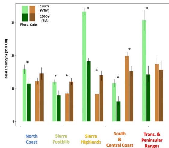
Fig. 4. Changes in basal area of oaks and pines between historical (1930s; VTM) and contemporary (2000s; FIA) forest surveys for five ecoregions of California. Asterisks denote change inferred between time periods based on nonoverlapping Bayesian 95% credible intervals (CRI).
