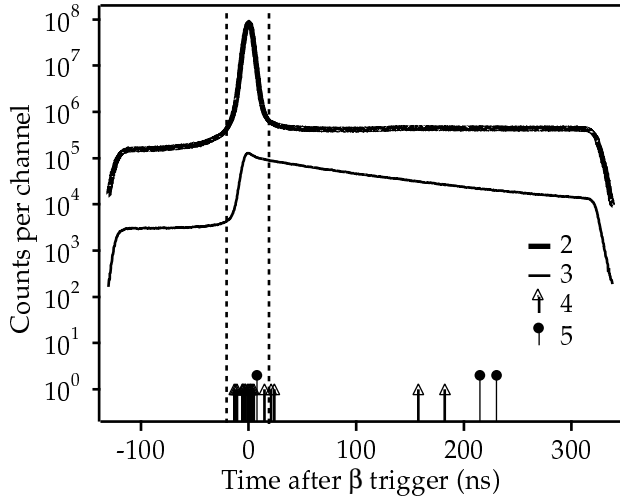
FIG. 1: Ps annihilation events passing all cuts as a function of time after the \beta decay ( t = 0 ). The dashed lines are at \pm 20 ns. 78% of the 3\gamma events have t > 20 ns, and 83% of the 2\gamma events occur within -20 < t < 20 ns. The TAC scaling for the horizontal axis is \approx 244 ps/channel. Five-photon counts have been offset for visibility.
