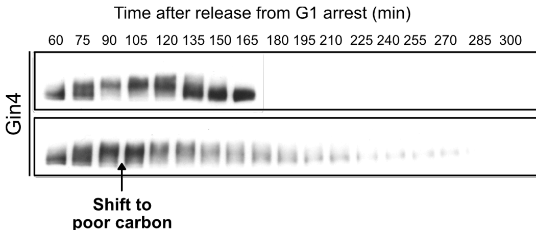
Figure 3.8. Mitotic dephosphorylation of Gin4 is delayed upon shift to poor carbon
