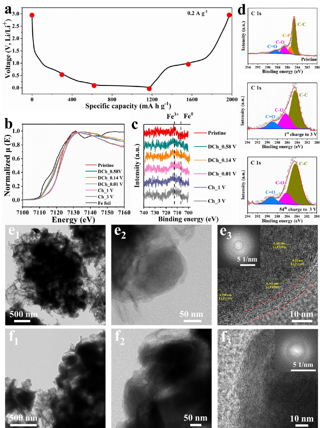
Figure 6. (a) First cycle voltage profile of FeP@CNs at 0.2 A g -1 . (b) Ex situ XAS of Fe K-edge at different states of (dis)charge. (c) Ex situ XPS of Fe 2p region at different states of (dis)charge. (d) Ex situ XPS of C 1s region at delithiated state in different cycles. TEM, HRTEM, and corresponding FFT images of FeP@CNs electrodes at different states: (e1–e3) first discharge and (f1–f3) first charge.
