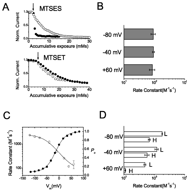
FIGURE 9. MTS modifications for the Y512C mutant. (A) Comparison of MTSES and MTSET modification rates at -80 mV (filled symbols) and +60 mV (open symbols). [Cl^-]_o was 4 mM to shift the fast-gate P_o - V curve to a technically convenient position so that the P_o at these two voltages significantly differs from each other. The horizontal axis represents the concentration (mM) \times cumulative exposure time (s). (B) Second order rate constants of MTSET modification at three voltages. [Cl^-]_o = 4 mM. The P_o s at these three voltages are: 0.20 ( -80 mV), 0.51 ( -40 mV), and 0.98 ( +60 mV). (C). Steady-state P_o - V curves (filled symbols) and the MTSES modification rates (open symbols) at 4 mM external Cl^- . Solid curves are drawn according to Boltzmann equations. (D) Comparison of the MTSES modification rates from the same voltage at different [Cl^-]_o . L: [Cl^-]_o = 4 mM. H: [Cl^-]_o = 142 mM. The P_o s at high [Cl^-]_o are: 0.60 ( -80 mV), 0.84 ( -40 mV), and 0.99 ( +60 mV). At all three voltages, the differences between low (L) and high (H) [Cl^-]_o are statistically significant. Note that at +60 mV, the difference in MTSES modification rates is significant even though the P_o values in the two conditions are both close to unity.
