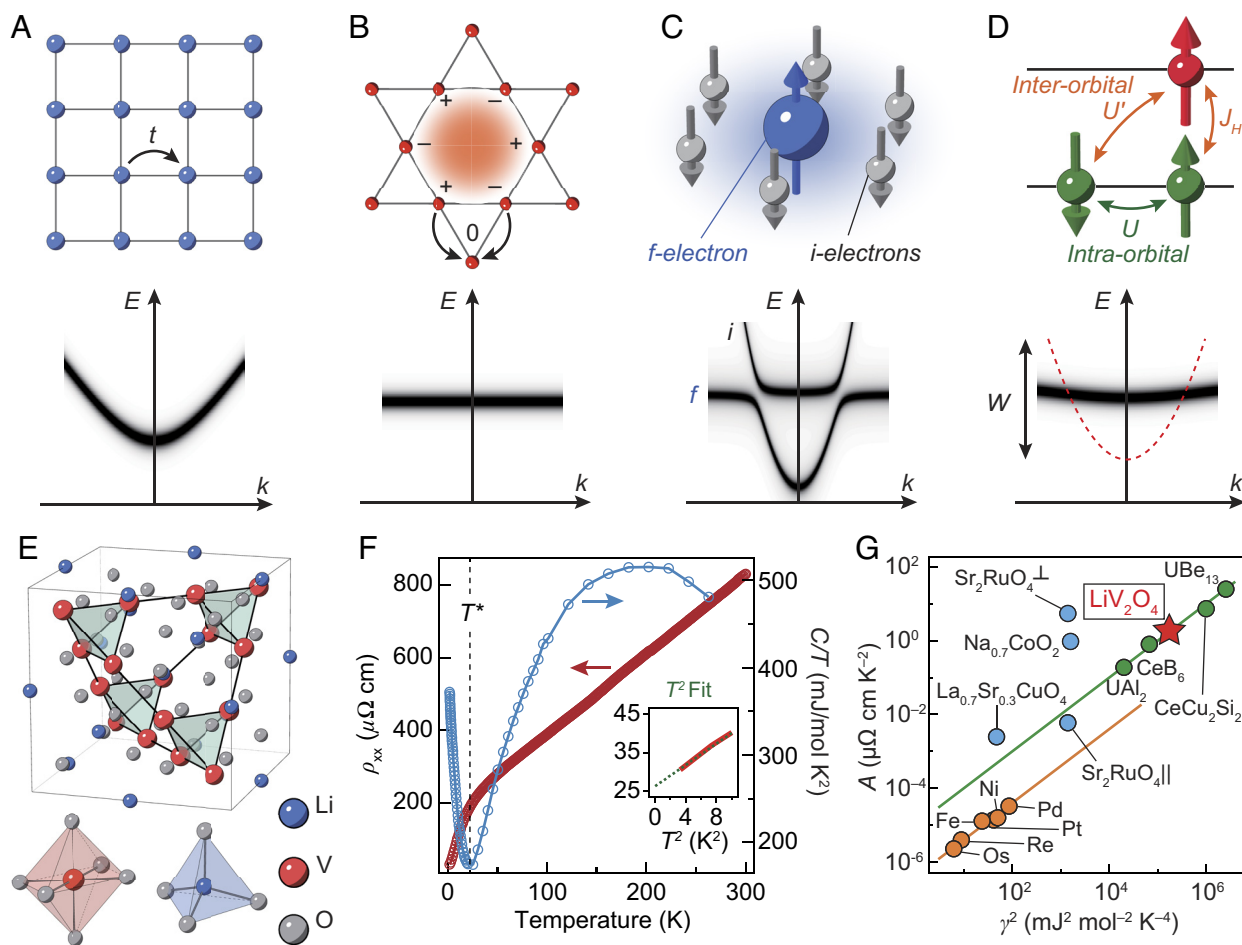
Fig. 1. Heavy fermion behavior of \text{LiV}_2\text{O}_4 . (A–D) Representative electronic band structures of the free electron model (A); flat band induced by geometrical frustration in the kagome lattice (B); hybridization between localized f -electron and itinerant electrons ( i -electrons) (C); and bandwidth renormalization induced by strong electron correlation via intraorbital Coulomb ( U ), interorbital Coulomb ( U' ), and Hund's coupling ( J_H ) (D). The red dashed curve corresponds to the bare band dispersion without electron correlations. (E) Crystal structure of \text{LiV}_2\text{O}_4 composed of \text{VO}_6 octahedra and \text{LiO}_4 tetrahedra. The V atoms form a frustrated pyrochlore network. (F) Heavy Fermi liquid behavior of \text{LiV}_2\text{O}_4 . The temperature-dependent electrical resistivity (red circles) shows a coherent-incoherent crossover while the electronic specific heat CT (blue circles) shows a large Sommerfeld coefficient \gamma \approx 420 \text{ mJ/mol K}^2 . The Inset shows \rho_{xx} versus T^2 plot (red) and T^2 fitting result (green). (G) The Kadowaki–Wood ratio of various materials, defined as the ratio of the coefficient of the T^2 term in electrical resistivity and \gamma^2 . \text{LiV}_2\text{O}_4 lies close to f -electron heavy fermion systems (green circles and line). Orange and blue circles represent the Kadowaki–Wood ratio of transition metals and oxide compounds, respectively. The value of the Kadowaki–Wood ratio was adapted from ref. 5.
