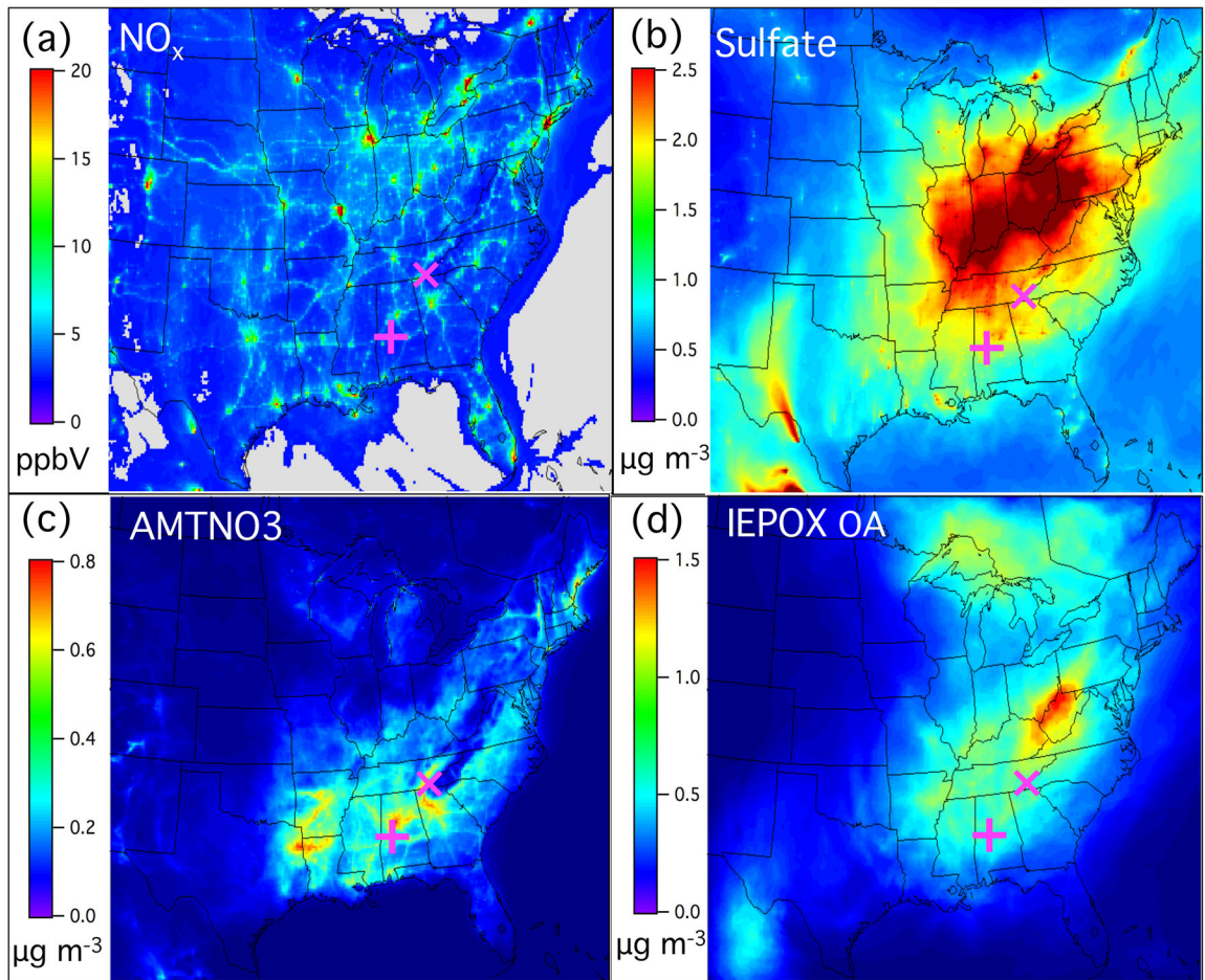
Figure 8. Spatial distribution of (a) \text{NO}_x , (b) sulfate, (c) monoterpene organic nitrate biogenic SOA, and (d) IEPOX related biogenic SOA in the Southeastern U.S. from the CMAQ model. “+” marks Centreville and “x” marks Look Rock.
