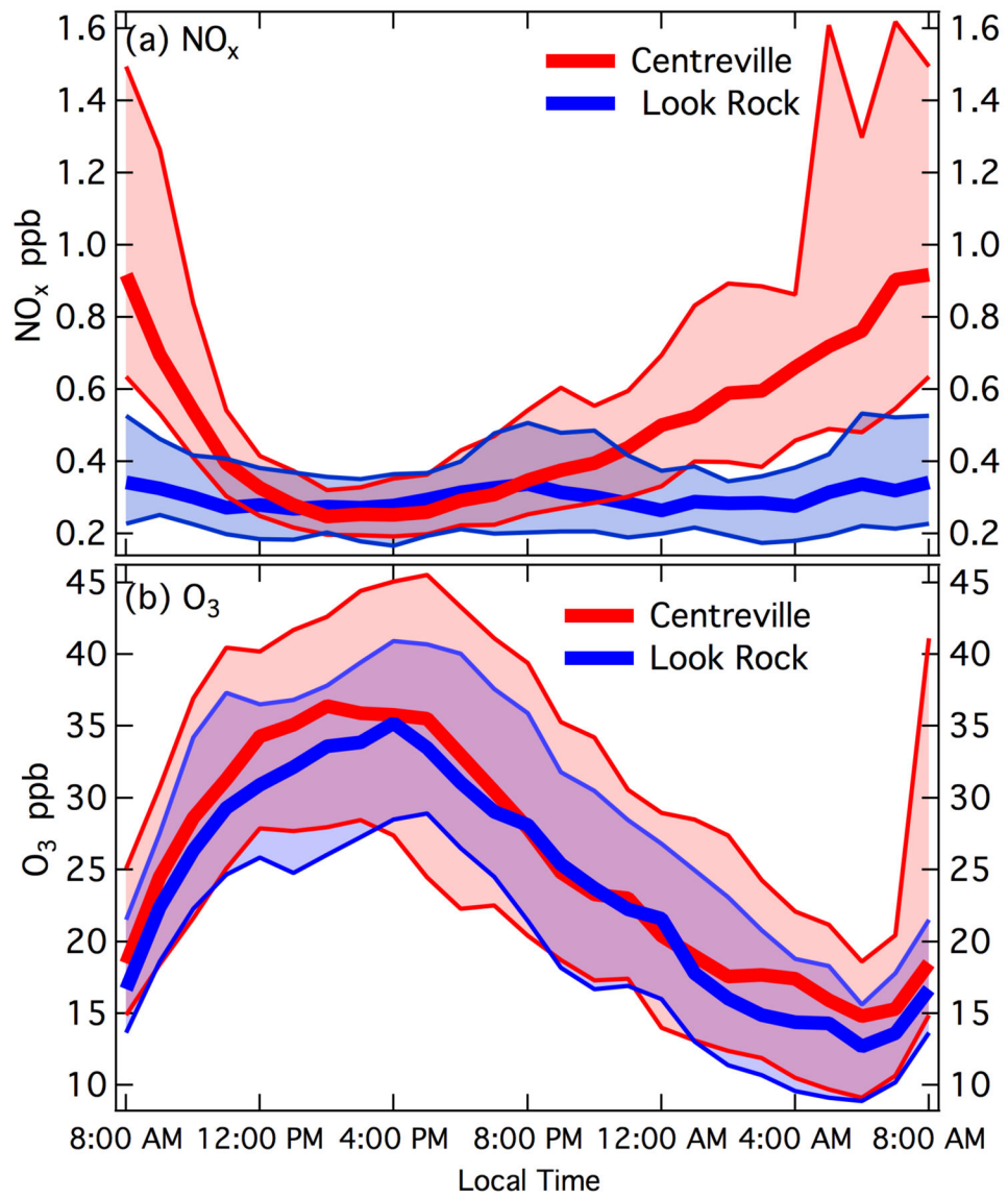
Figure 4. Diurnal plot of (a) NO x and (b) O 3 at both sites. Medians, 25th percentiles and 75 percentiles are shown on the figure.
