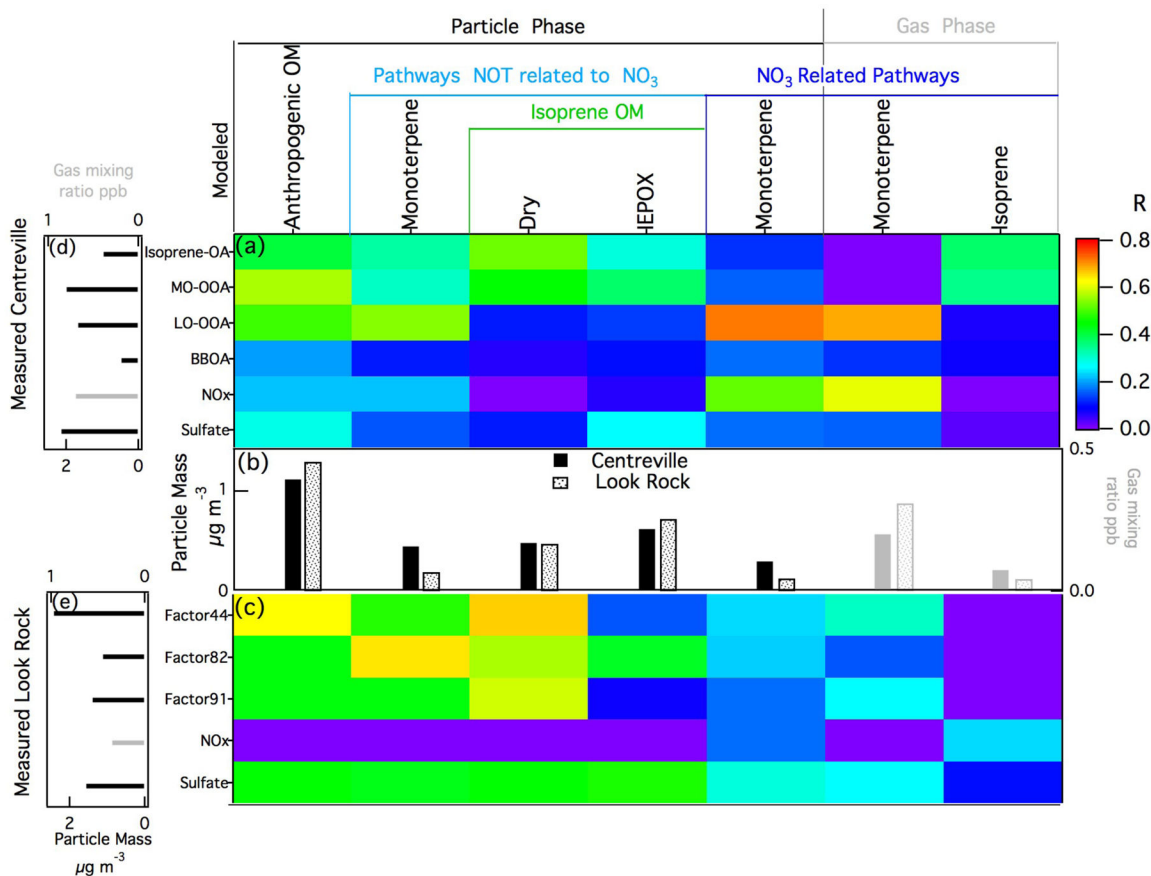
Figure 7. Average concentration of CMAQ modeled species and heat map of correlation coefficients of CMAQ model species to measurements at (a) CTR and (c) LRK. Low 24-hour significance level pairs ( P > 0.05 ) are shaded. (b) Concentrations of CMAQ modeled species. Concentrations of measured species at (d) CTR and (e) LRK. Details of the modeled species can be found in Text S3 and Table S7. Low concentration species ( < 0.05 \mu\text{g m}^{-3} ) are excluded in this figure.
