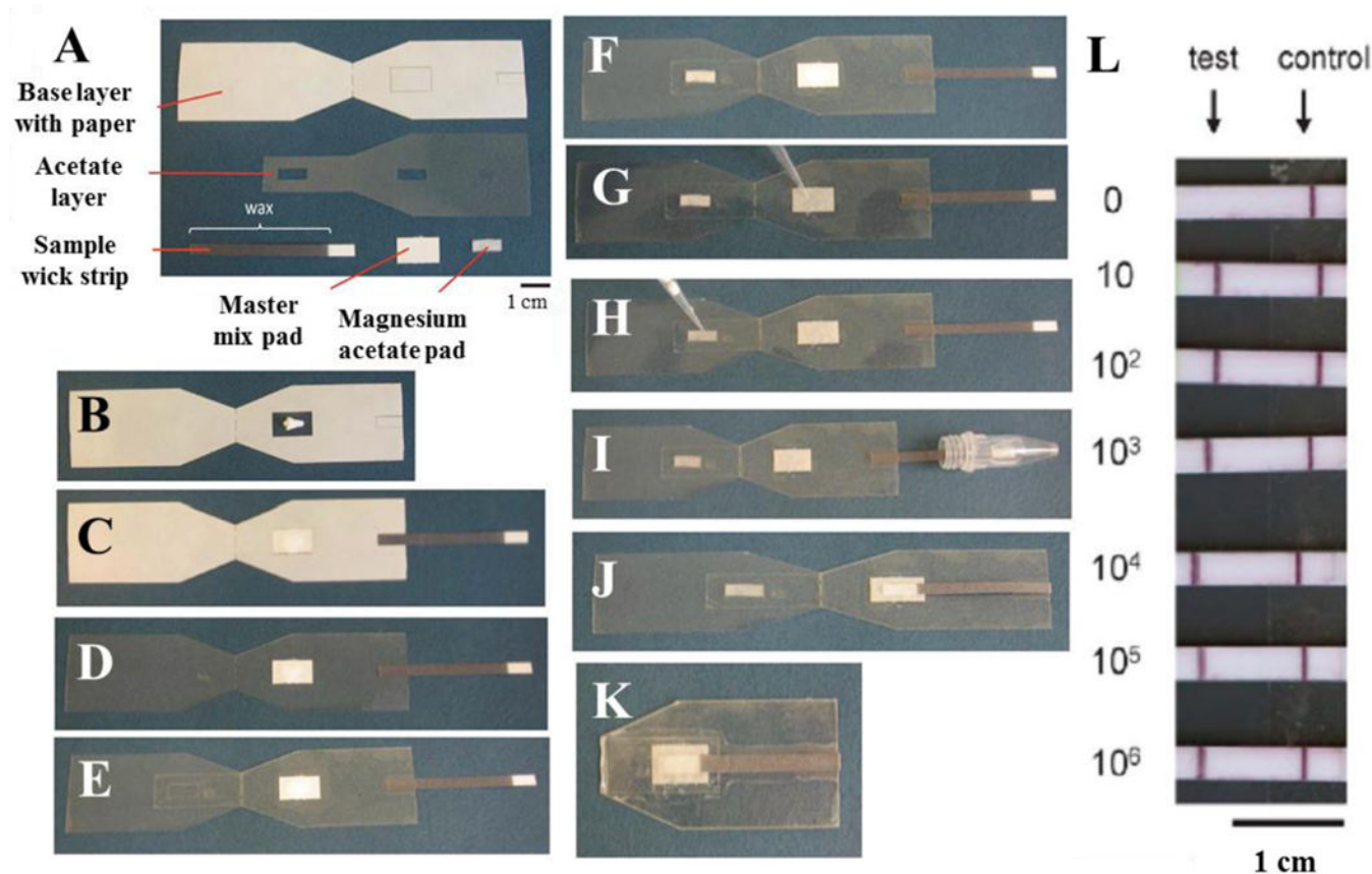
Fig. 6. Paper-based viral load detection system to perform recombinase polymerase amplification of HIV DNA, system assembly and operation
