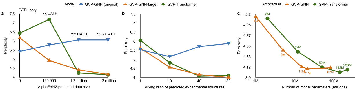
Figure 3.6: Ablation studies on training data. (a) Effect of increasing the number of predicted structures. The original GVP-GNN degrades with training on additional data, but GVP-GNN-large and GVP-Transformer improve with increasing numbers of predicted structures. (b) Effect of increasing the mixing ratio during training between predicted and experimental structures. A higher ratio of predicted structures improves performance for both GVP-GNN-large and GVP-Transformer. (c) GVP-GNN and GVP-Transformer model size.
