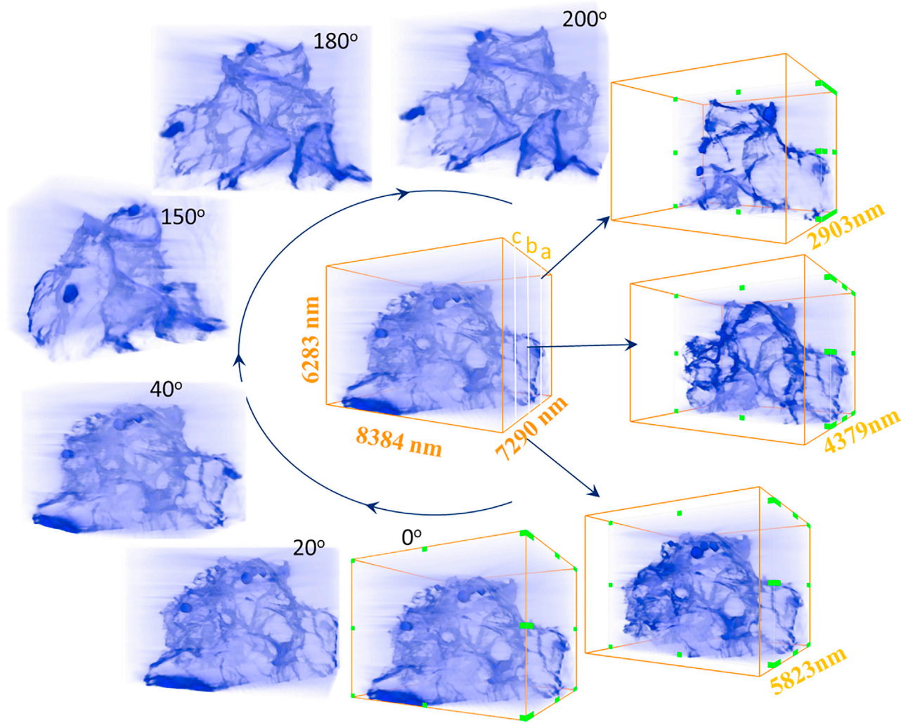
Figure 4. STEM tomography reconstructed the 3D image of the SEI husk after Li stripping, illustrating the hollow, crumpled SEI structure
