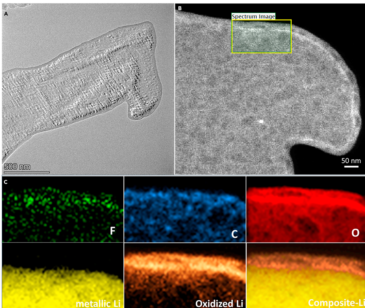
Figure 6. The morphology of a new Li electrode after two lithiation cycles (the empty husks are reinflated by the newly plated Li) (A) Cryo-TEM and (B) cryo-STEM image of the second round of plated Li metal. (C) Elemental maps of F, C, O, metallic Li, oxidized Li, and composite Li map in the rectangular spectrum image region in (B).
