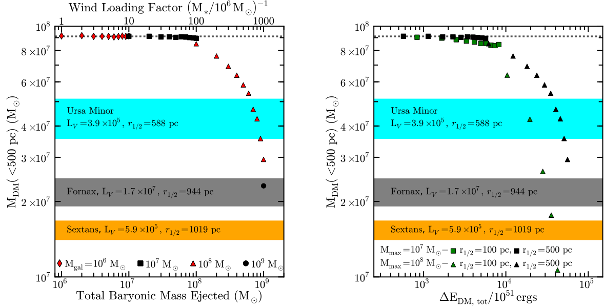
Figure 4.5: Left : The mass remaining within 500 pc after repeated blowouts of a galaxy with M_{\text{max}} = 10^6, 10^7, 10^8 , and 10^9 M_{\odot} , all with r_{1/2} = 500 \text{ pc} , as a function of mass blown out. Right : The mass remaining after blowouts of 10^7 M_{\odot} and 10^8 M_{\odot} with either r_{1/2} = 100 \text{ pc} (in green) or 500 \text{ pc} (in black) as a function of the cumulative change in the dark matter energy. The dotted line indicates the original mass within 500 pc, and the colored bands indicate the dark matter within 500 pc for Ursa Minor, Fornax, and Sextans. As the stellar component of Fornax contributes non-negligibly to the mass near its center, we have subtracted 7 \times 10^6 M_{\odot} from the dynamical mass in order to account for the stellar mass within 500 pc for this galaxy (Jardel & Gebhardt, 2012). More than several times 10^8 M_{\odot} must be ejected to bring the mass into agreement with Ursa Minor (though each blowout may be \sim 10^8 M_{\odot} ), and the requisite energy also exceeds the total supernovae budget for six of the nine classical dSphs. Furthermore, we note that \Delta E_{\text{DM}} is a lower limit on the energy that must be injected, as it does not account for energy escaping via radiation or the energy required to eject the baryons.
