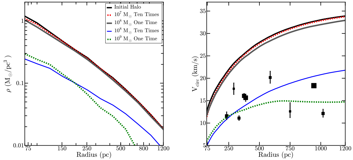
Figure 4.4: The density (left) and circular velocity (right) profiles of the halo after ten blowouts of 10^7 M_\odot and one blowout of 10^8 M_\odot (upper lines; as illustrated in Figure 4.3), and after ten blowouts of 10^8 M_\odot and one blowout of 10^9 M_\odot (lower lines), all with r_{1/2} = 500 pc (the qualitative results are similar for r_{1/2} = 100 pc). Removing 10^7 M_\odot ( 10^8 M_\odot ) ten times is less effective at removing dark matter from the inner region of the halo than removing 10^8 M_\odot ( 10^9 M_\odot ) once. Furthermore, note that \sim 10^9 M_\odot of baryons must be removed from the galaxy – though it does not have to leave the halo – to bring the circular velocity into agreement with the data.
