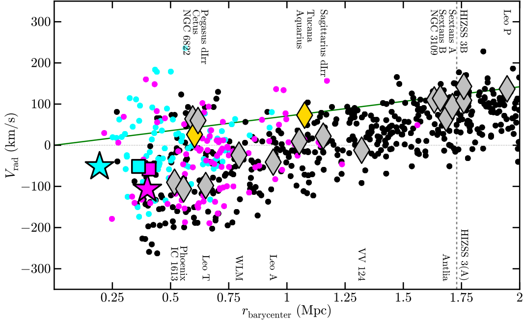
Figure 2.15: Barycentric radial velocity versus barycentric distance for Local Group galaxies compared to expectations from the Zeus & Hera simulation. The centers of Zeus (cyan) and Hera (magenta) are indicated by large stars, while M31 (cyan) and the MW (magenta) are shown by squares. All halos with M_\star > 3 \times 10^3 M_\odot and beyond 300 kpc of either Zeus or Hera are plotted as circles. Large diamonds indicate known galaxies in the Local Group beyond 300 kpc of either giant. Backsplash halos of Zeus are shown as cyan while those that have interacted with Hera are plotted in magenta. The black points are halos that have yet to be accreted by either host. The grey diamonds mark LG galaxies that have gas while the yellow diamonds correspond to Cetus and Tucana, two gas-free dwarf that are good backslash candidates. For reference, the green line shows the asymptotic linear Hubble relation for our simulated cosmology.
