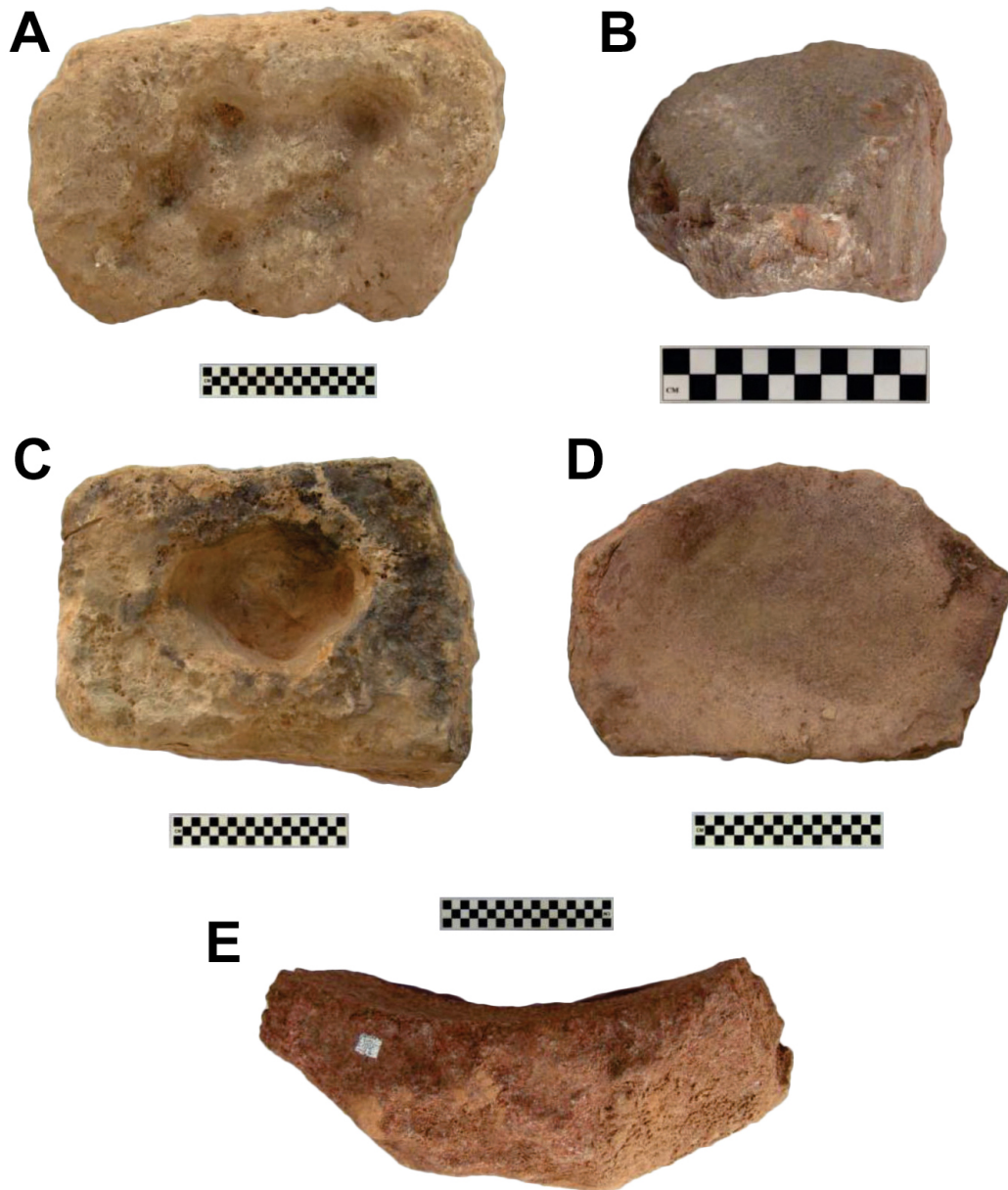
Figure 12. Selected netherstones from Khirbat en-Nahas, 2006 excavations. A, anvil, Area T, Locus 1519; B, small dimpled anvil, Area R, Locus 1804; C, mortar, Area T, Locus 1511; D, grinding slab, Area T, Locus 1523; E, saddle quern, Area T, Locus 1507. Individual squares in the scale bars are 1 cm wide.
