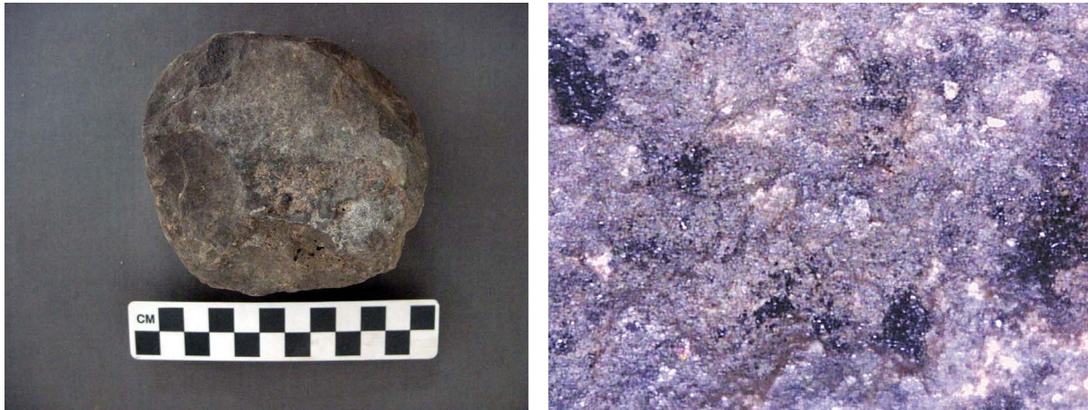
Figure 13. Dimpled hammerstone from Khirbat en-Nahas; andesite rock. Photomicrograph (right) of centre of 'dimple' shows crushed rock grains, pits, loose rock particles, and 'frosted' appearance. Image width = 2 mm.
