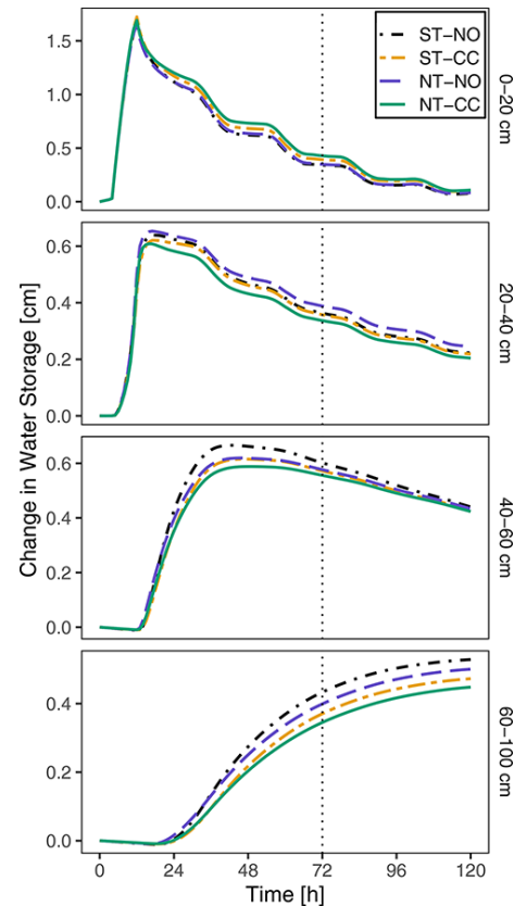
Figure 8. Change in water storage across soil layers (treatment means). The gray, dotted vertical line indicates day 3 after irrigation.
