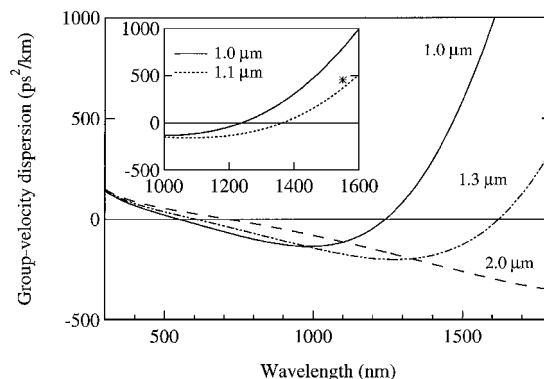
Fig. 1. Calculated GVD for 1.0-, 1.3-, and 2.0- \mu\text{m} -diameter waist tapered fibers. The inset shows the GVD of the 1.0- and 1.1- \mu\text{m} waist tapers in proximity to their second ZDWs, and the asterisk shows the dispersion value measured at 1550 nm.
