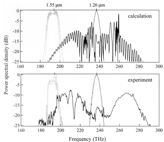
Fig. 2. Comparison of numerical simulations (top) and experimental results (bottom) for 750-pJ, 80-fs pulses at 1.26 \mu\text{m} (darker curves) and 350-pJ, 100-fs pulses at 1.55 \mu\text{m} (lighter curves). The input spectra are shown as dotted curves.
