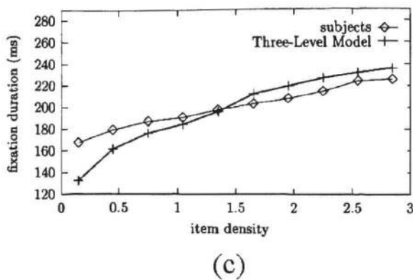
Figure 3: Results of the computer simulation: (a) example scan path, (b) RT histogram, (c) FD as a function of item density, (d) SF as a function of item density
