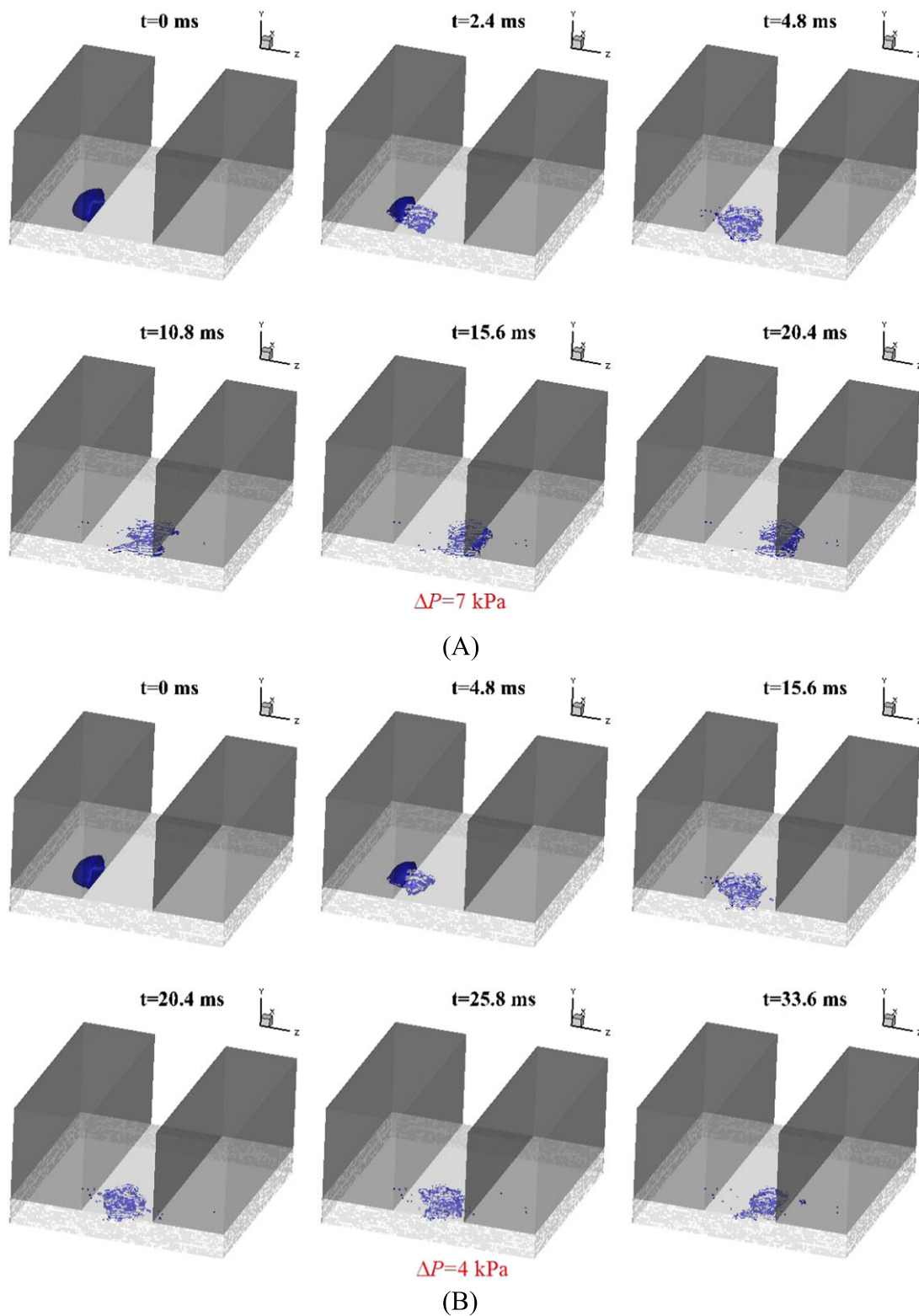
FIGURE 7 Iso-surface of liquid water phase fraction \gamma = 0.5 in cases with different \Delta p . (A) \Delta p = 7 kPa, \theta_f = 90^\circ ; (b) \Delta p = 4 kPa, \theta_f = 90^\circ [Colour figure can be viewed at wileyonlinelibrary.com]
