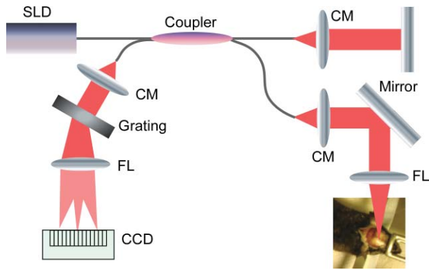
Fig. 2 Schematic of the OCT system (FL, focusing lens; DG, diffraction grating; CM, collimator; LSC, line-scan camera; SLD, superluminescent diode).
