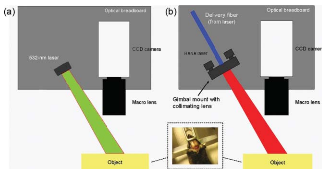
Fig. 1 Experimental setup of (a) photocoagulation by a 532-nm green laser and (b) laser speckle imaging by a HeNe laser. The insert shows an intact C3H mouse skull with the scalp removed.
