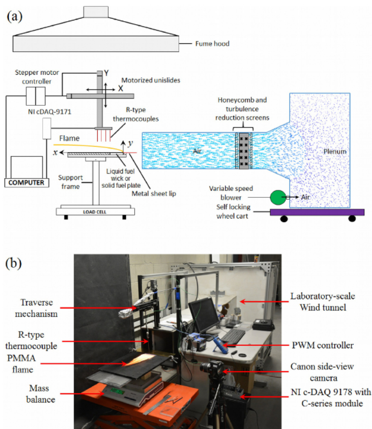
Figure 1. Experimental Setup. (a) Schematic of the experimental setup used to measure mass-loss rates and temperature profiles over a forced-convection boundary layer diffusion flame. (b) Experimental setup for investigating boundary layer diffusion flames under forced flow. Please click here to view a larger version of this figure.
