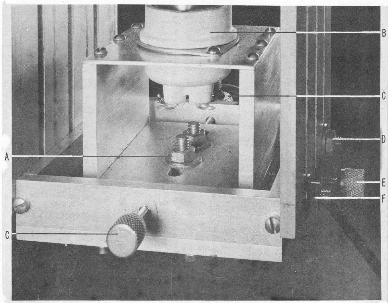
Fig. 11. Light-source support. (A) Transverse locking screws. (B) Arc tube socket. (C) Transverse positioning screws. (D) Vertical locking screw. (E) Longitudinal positioning screw. (F) Vertical locking screw.
