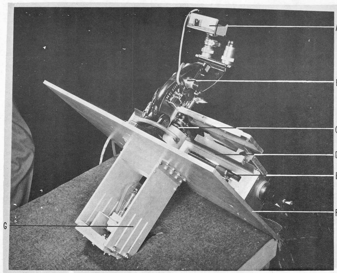
Fig. 15 Alpha-track counter, bottom view. (A) Photomultiplier housing. (B) Microscope. (C) Dark-field adapter and modulation system. (D) Scanner. (E) Scanner carriage split nut. (F) Base plate. (G) Light-source housing.
