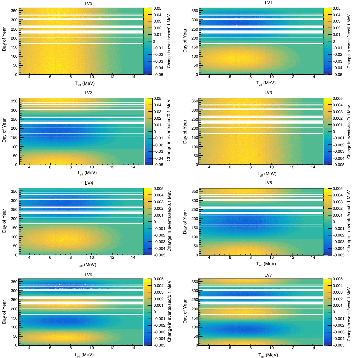
FIG. 4. The eight signal types expected in SNO if a_{\text{SNO}}^{(3)} = 0.01 \text{ GeV}^{-1} and c_{\text{SNO}}^{(4)} = 10 \text{ GeV}^{-2} . The figure was generated by taking the {}^8\text{B} CC and ES Monte Carlo events for the selected runs in Phases I and II and weighing each event by the correction to the survival probability, then normalizing by the livetime. White areas denote days for which there was no livetime. LV0, LV1, and LV2 are proportional to E , while the other signals are proportional to E^2 , and can therefore be seen to be shifted slightly toward higher energies.
