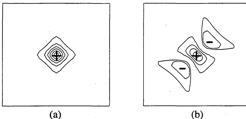
Figure 4.1 Pure-Absorption mode and Mixed-Phase 2D NMR Spectra. Spectrum (a) is an example of a pure-absorption mode line with equal homogeneous broadening in both dimensions. Spectrum (b) is an example of a mixed-phase line with the same parameters. Note in (b) the presence of both positive (+) and (-) contours, giving a peak of much larger effective linewidth.
