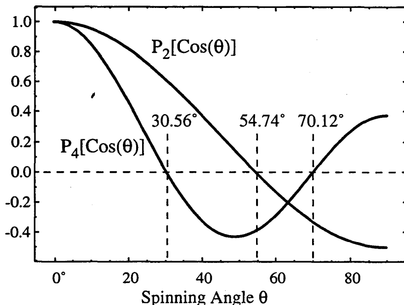
Figure 3.1 2nd and 4th Order Legendre Polynomials. There is no single angle at which both the 2nd and 4th order polynomials are zero. Therefore, multiple angles will be needed to average the second-order quadrupolar interaction (equation. 3.1).
