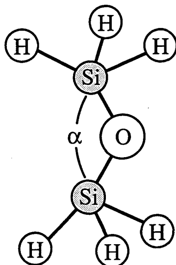
Figure 8.9 Electric Field Gradient Model Compound;. The molecule \text{H}_3\text{Si-O-SiH}_3 may be used as a rough model to show the relative sizes of the EFG tensor as the Si-O-Si bond angle is changed.
