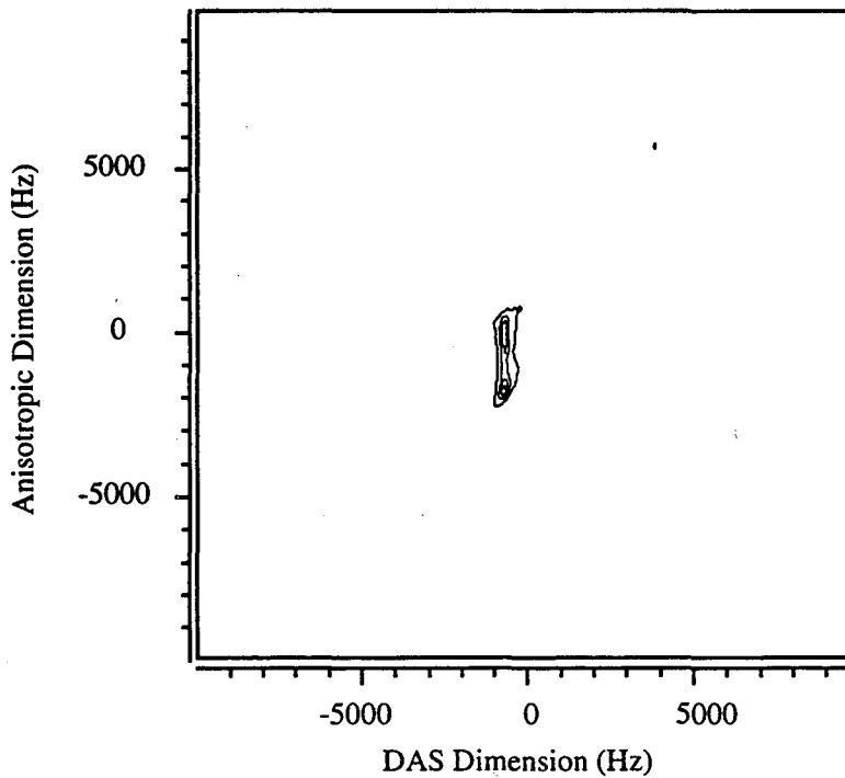
Figure 4.9 Hypercomplex DAS Spectrum. This spectrum was taken with the pulse sequence given in figure 4.3.
