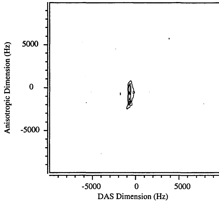
Figure 4.8 Echo DAS Spectrum. This spectrum was taken with the pulse sequence given in figure 4.3.
