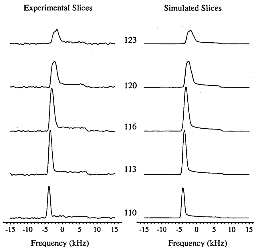
Figure 8.8 \text{SiO}_2 Anisotropic Slices and Simulations. Five of the slices which were simulated in table 8.3 are shown along with the best fit. The slice number in the isotropic peak which they were extracted from is indicated.
