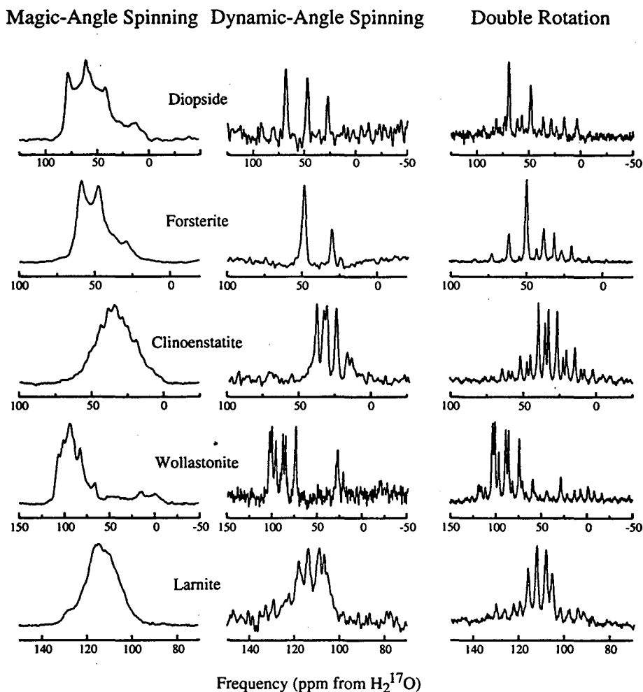
Figure 8.2 Crystalline 9.4T DAS, DOR and MAS Spectra. The MAS spectra are very similar to those observed by Timken et al. 150 and all spectra are shown with permission from the thesis by Mueller. 15 The MAS and DOR spectra were taken with standard one-pulse experiments while for the DAS spectra the original DAS pulse sequence was used.
