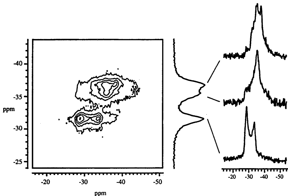
Figure 7.6 \text{RbNO}_3 9.4T 2D MAS detected DAS Contour Plot. Single site MAS slices through each isotropic peak in the DAS dimension have been extracted and are displayed to the right of the contour plot.
