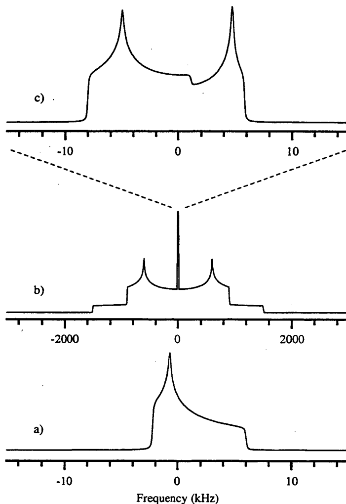
Figure 2.5 Static CSA (a), 1st Order (b) and 2nd Order (c) Quadrupolar Lineshapes. For the chemical shift anisotropy simulation, \omega_l was 100 MHz, \delta_{iso,cs} was 10 ppm, \delta^{CS} was 50 ppm and \eta_{CS} was 0.3. For the 1st Order and 2nd Order Quadrupolar lineshapes the \omega_l was 100 MHz, \delta_{iso,cs} was 10 ppm, I was 3/2 , \omega_Q was 3.0 MHz, \eta_Q was 0.2.
