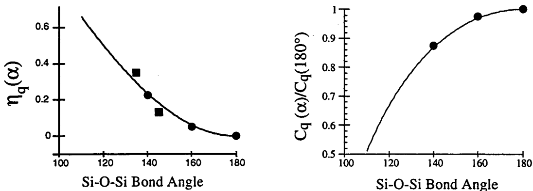
Figure 8.10 Ab Initio Quadrupolar Parameters for \text{H}_3\text{Si-O-SiH}_3 . The quadrupolar coupling constant and asymmetry parameter were calculated using Gaussian algorithms for the angles 180^\circ , 160^\circ and 140^\circ . Circles indicate values calculated by Tossell and Lazzeretti while square are experimental points from Stebbins et al.
