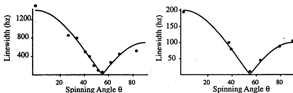
Figure 3.14 Homonuclear Dipolar Linewidth versus Spinning Angle. The left set corresponds to \text{Na}_2\text{C}_2\text{O}_4 ^{23}\text{Na} linewidth as a function of angle where the static linewidth is 1400 Hz. The right set corresponds to \text{RbClO}_4 ^{87}\text{Rb} linewidth as a function of angle where the static linewidth is 195 Hz.
