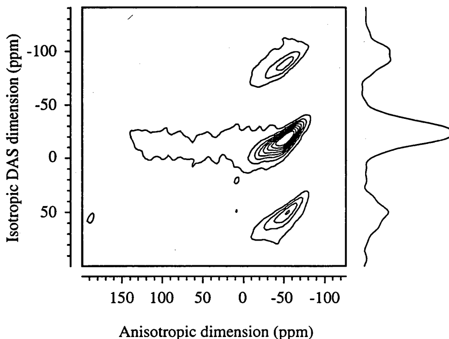
Figure 8.7 2D DAS Spectrum of Amorphous SiO 2 . The isotropic dimension shows a single broad peak with spinning sidebands on both sides. The anisotropic slices are seen to increase in asymmetry parameter and decrease in quadrupolar coupling as the isotropic shift gets larger.
