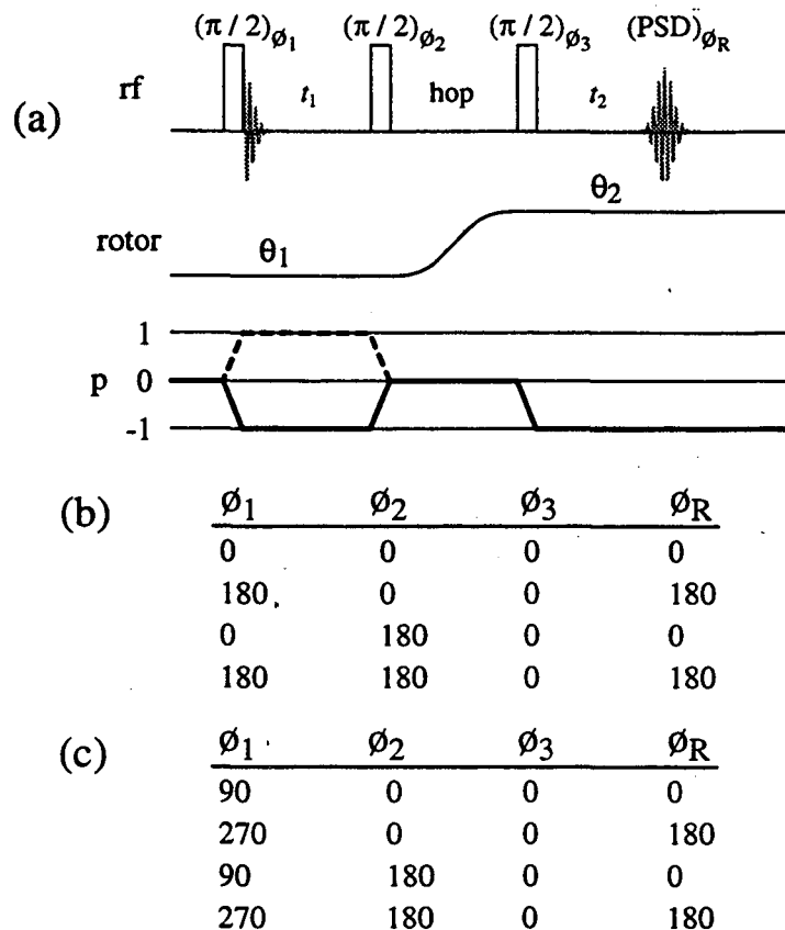
Figure 4.4 Hypercomplex DAS Experiment. The pulse sequence (a), coherence pathway, and phase cycle are given above. Cycle (b) is the cosine data set and cycle (c) is the sine data set.
