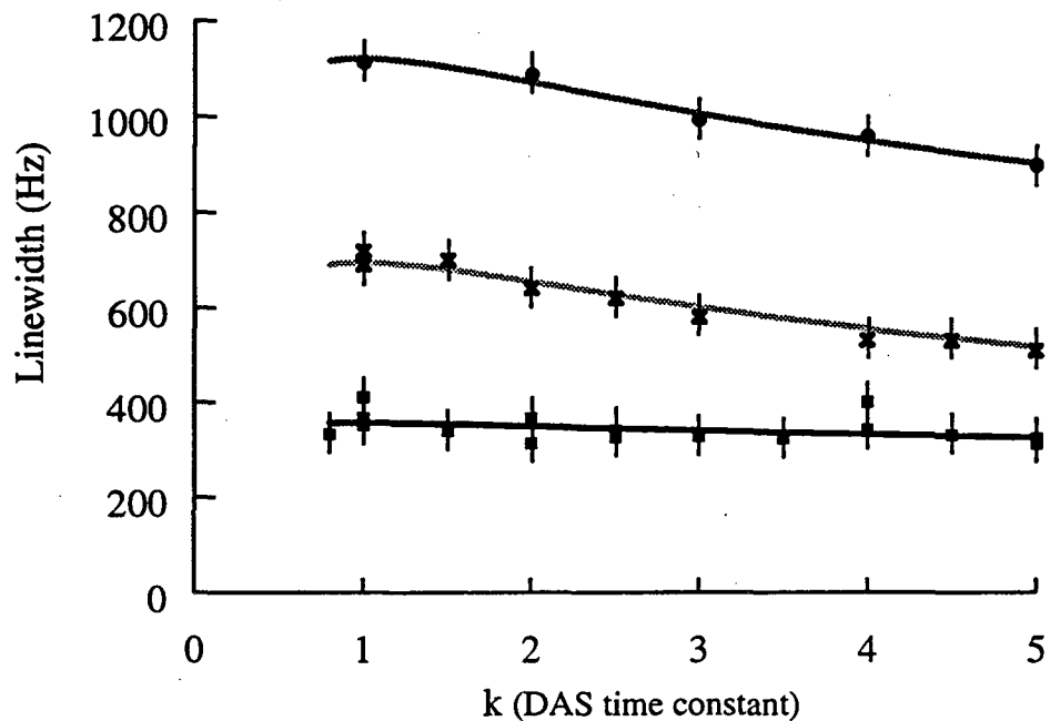
Figure 3.15 Dynamic-Angle Spinning Linewidths as a function of k . The solid circles are for D_3BO_3 , the crosses are for Na_2C_2O_4 and the solid boxes are for RbClO_4 . The lines through each set of points are the best fit with the linewidth function given by equation 3.39.
