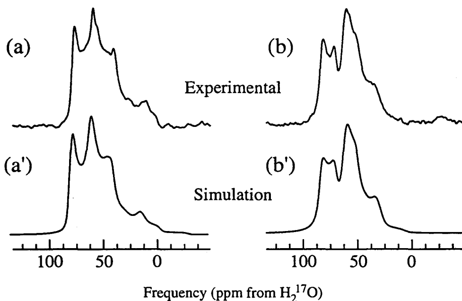
Figure 8.4 Crystalline Diopside 9.4T and 11.7T MAS Spectra. The MAS spectra at 9.4T (a) are shown as well as at 11.7T (b). All spectra are shown with a ppm scale referenced relative to H_2^{17}O . The simulations (a' and b') were performed with the isotropic chemical shift and quadrupolar product parameters fixed to those in table 8.1. The simulation results are given in table 8.2.
