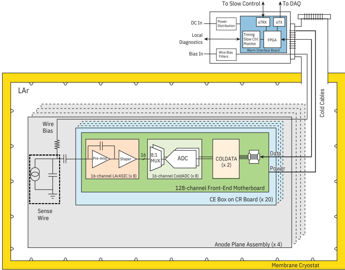
Figure 1. Schematic of the TPC electronics readout chain for ProtoDUNE-HD. The DUNE HD far detector uses the same design, scaled up to 150 APAs. The APA sense wires are represented on the left as an equivalent current source for electron signals from the TPC and equivalent capacitance. Their signals are connected to the front end of LArASICs through a physical capacitor. The LArASIC, ColdADC, and COLDATA ASICs are described in further detail in section 3. The ASICs are arranged onto front-end motherboards, which are described in section 4. These motherboards are contained within cold electronics (CE) boxes, which are plugged into capacitive-resistive (CR) boards on the APA [10]. The interface to all external systems is managed by warm interface boards shown on top of the cryostat, which are described in section 5.
