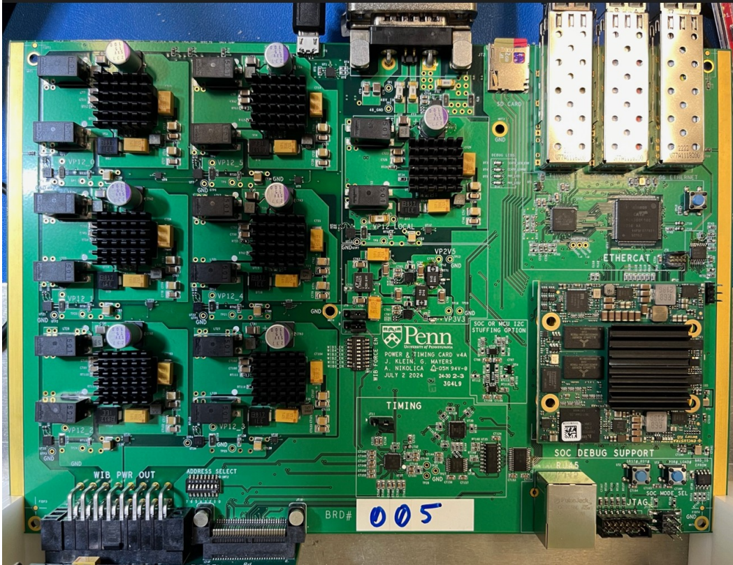
Figure 17. Revised PTC containing new functions relative to the ProtoDUNE-HD PTCs. The connections to the PTB are through the connectors shown in the bottom left, and front panel connections to external systems are at the top.
