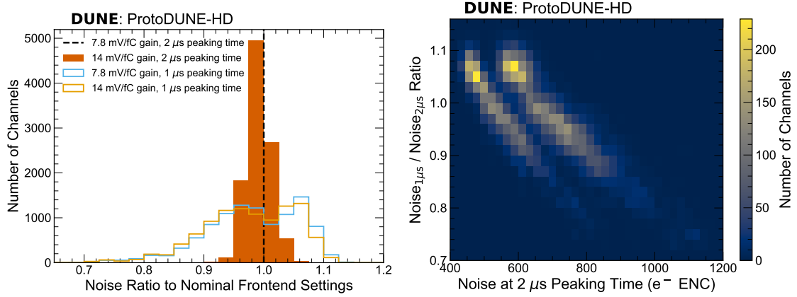
Figure 27. Left: ratios of noise levels per channel for settings of 7.8 or 14 mV/fC gain and 1 or 2 \mu s peaking time in the LArASIC. Comparisons are against the nominal settings, which were 7.8 mV/fC gain and 2 \mu s peaking time. Right: ratio of noise at 7.8 mV/fC gain with 1 \mu s peaking time to noise with 2 \mu s peaking time, plotted against noise with the nominal settings. Typical channels have slightly worse noise with 1 \mu s peaking time, but channels in the higher noise tail are improved with 1 \mu s peaking time.
