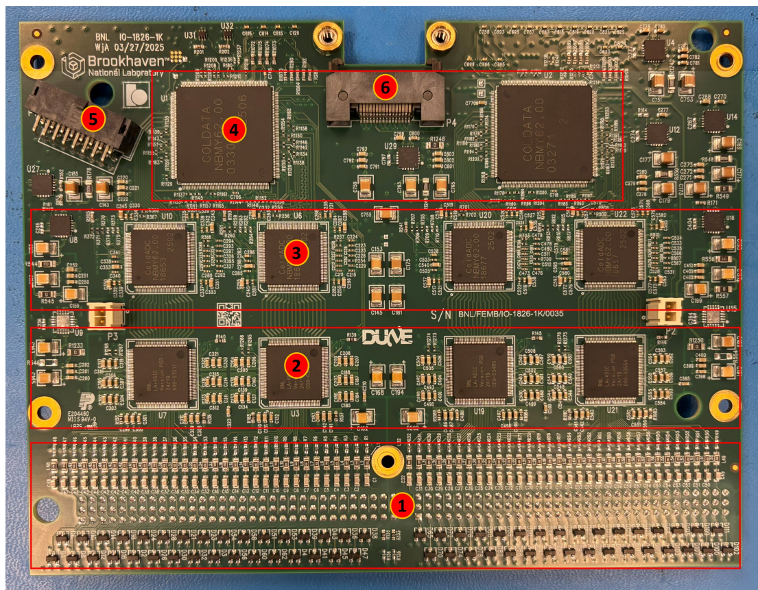
Figure 7. Picture of the top layer of a FEMB. The locations of input connectors and protection diodes (1), four LArASICs (2), four ColdADCs (3), two COLDATAs (4), the Samtec IPL1 connector for power (5), and the Samtec ASP 36-pin data connector (6) are indicated. Note that another four LArASICs and four ColdADCs are placed on the other side of the PCB, directly opposite the ones that are shown.
